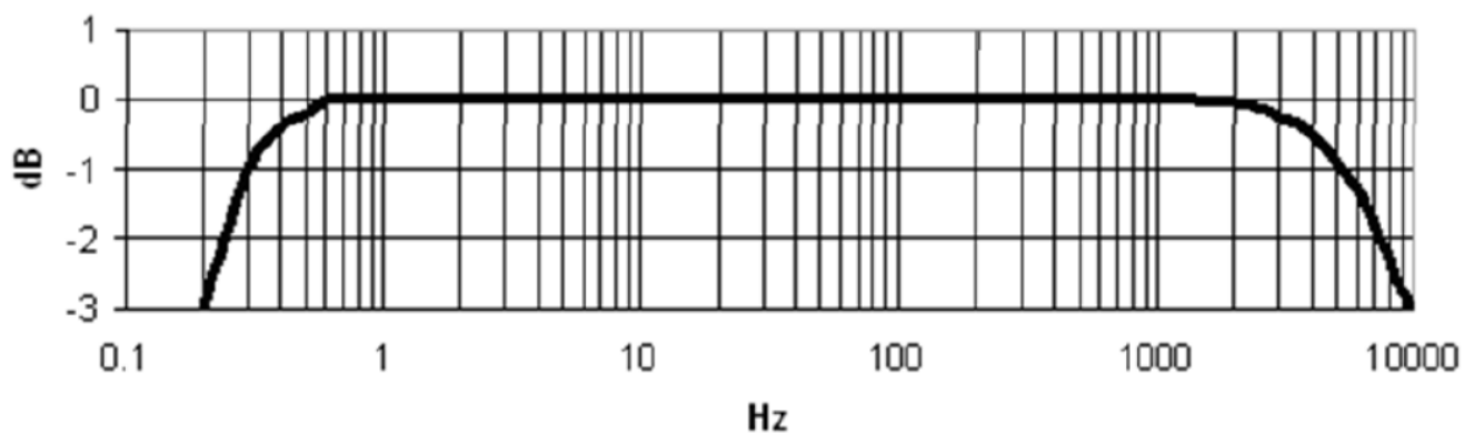
Figure 5: 200355 Accelerometer Frequency Response
