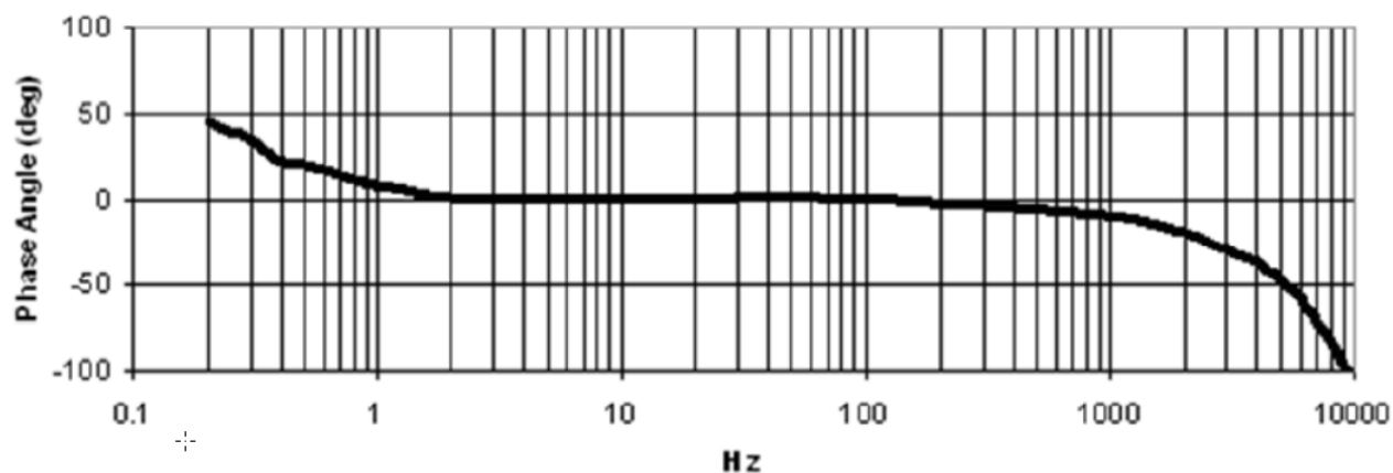
Figure 6: 200355 Accelerometer Phase
