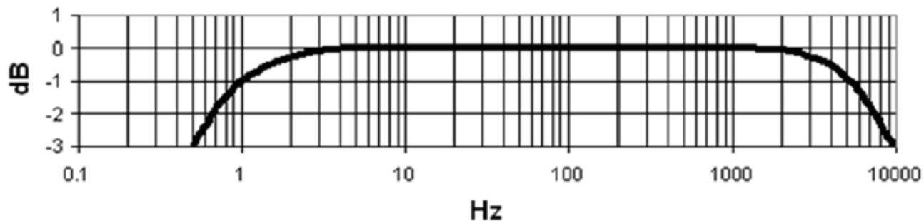
Figure 3: 200350 Accelerometer Frequency Response
