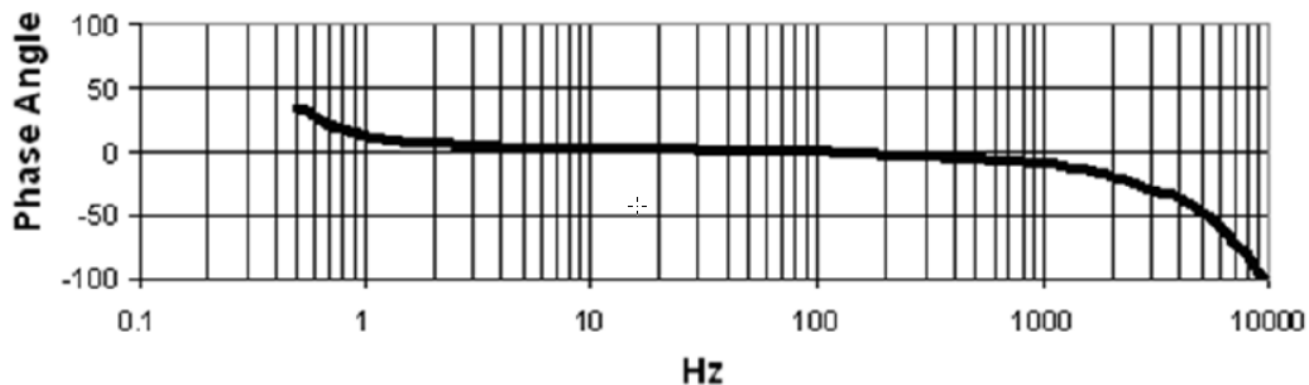
Figure 4: 200350 Accelerometer Phase
