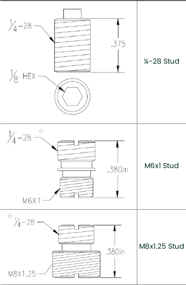
Figure 8: Mounting Stud Dimensional Drawings
