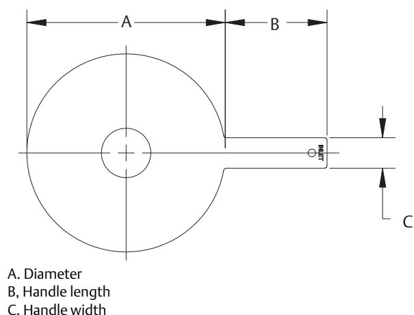
Figure 48. Rosemount1495PC Paddle Type Orifice Plate (DIN, Paddle, Square Edged, Concentric)
