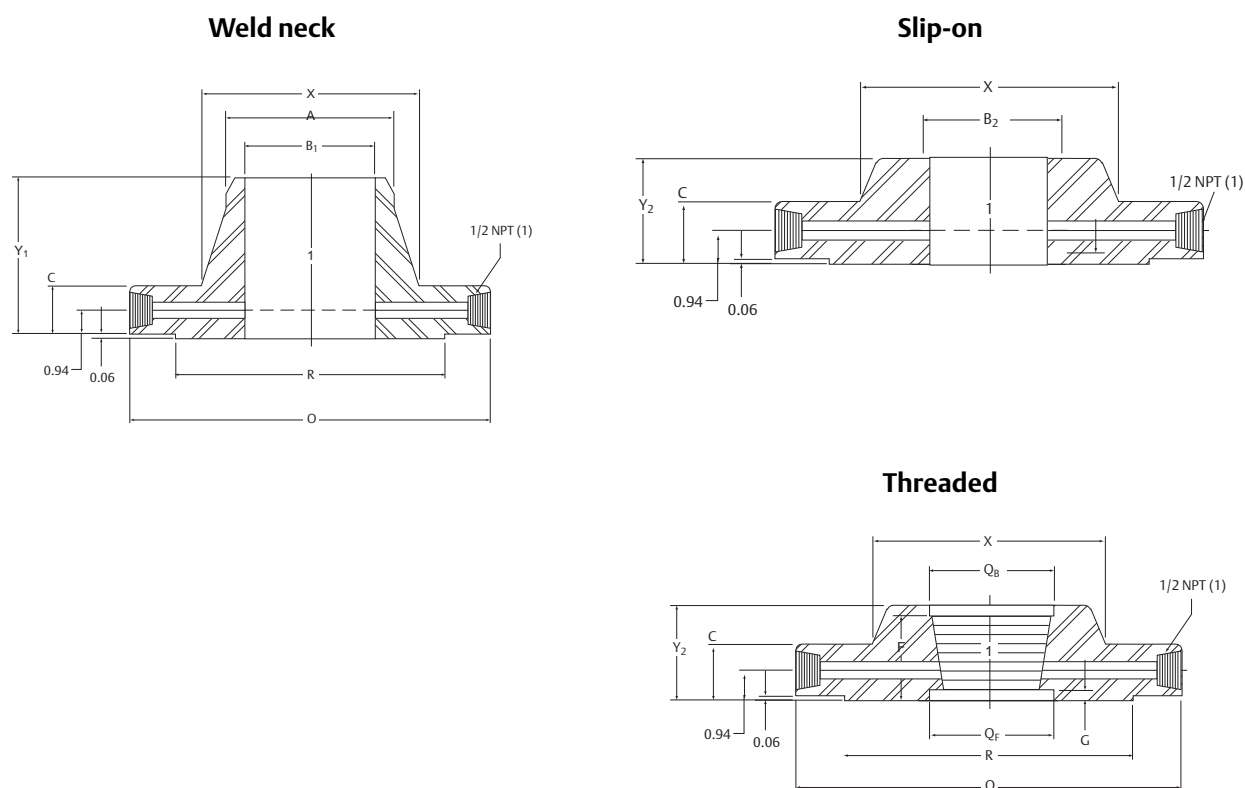
Figure 51. Class 300
