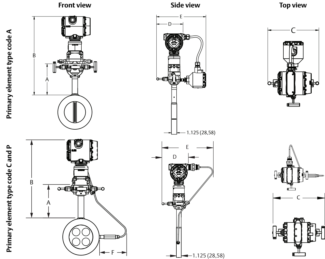
Figure 18. Rosemount 3051SFC Compact Flowmeter
