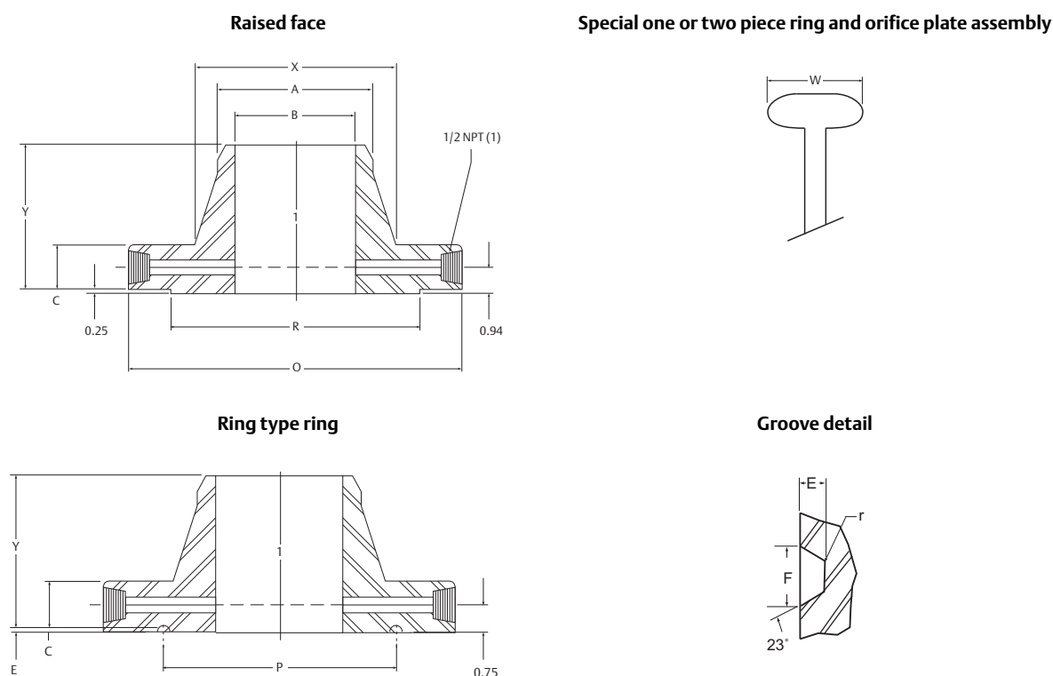
Figure 52. Class 600, 900, 1500, and 2500
