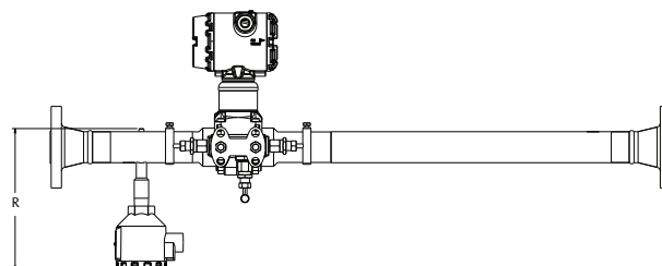
Temperature sensor
