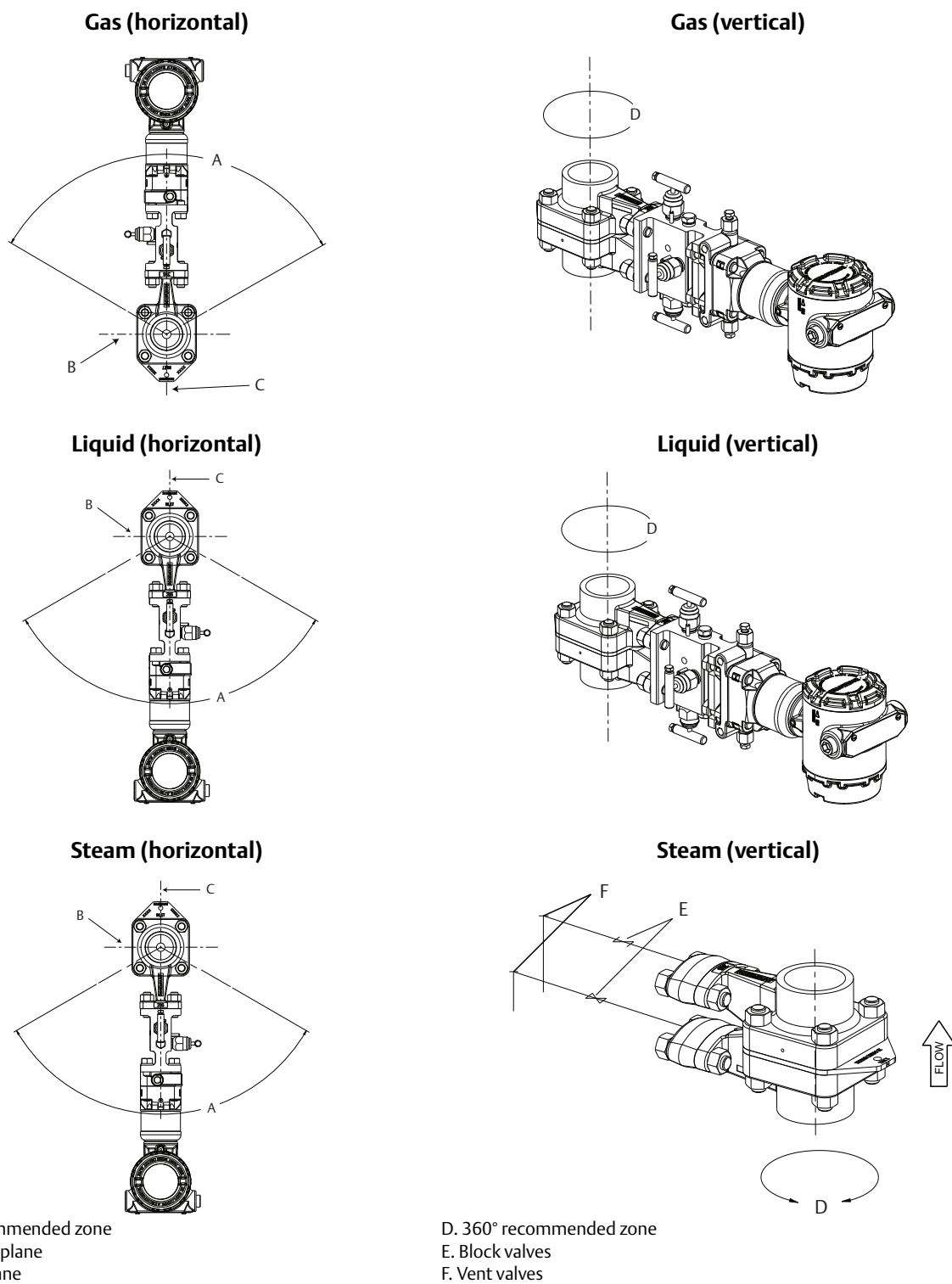
Figure 12. Rosemount 1195 Flowmeter Orientation with H-Pattern Manifold (Recommended)
