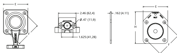
Figure 46. Enhanced Body Support Orifice plate
