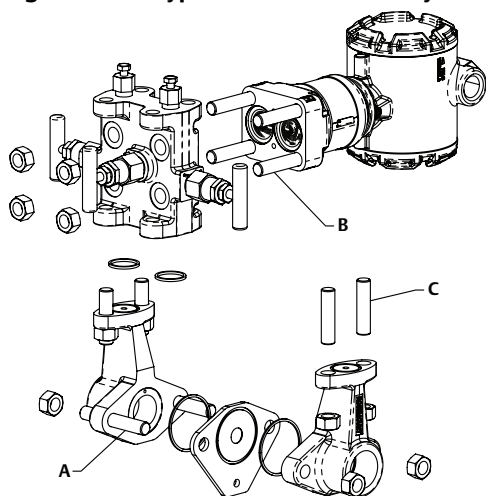
Figure 2. Bolt Types for Traditional Body
