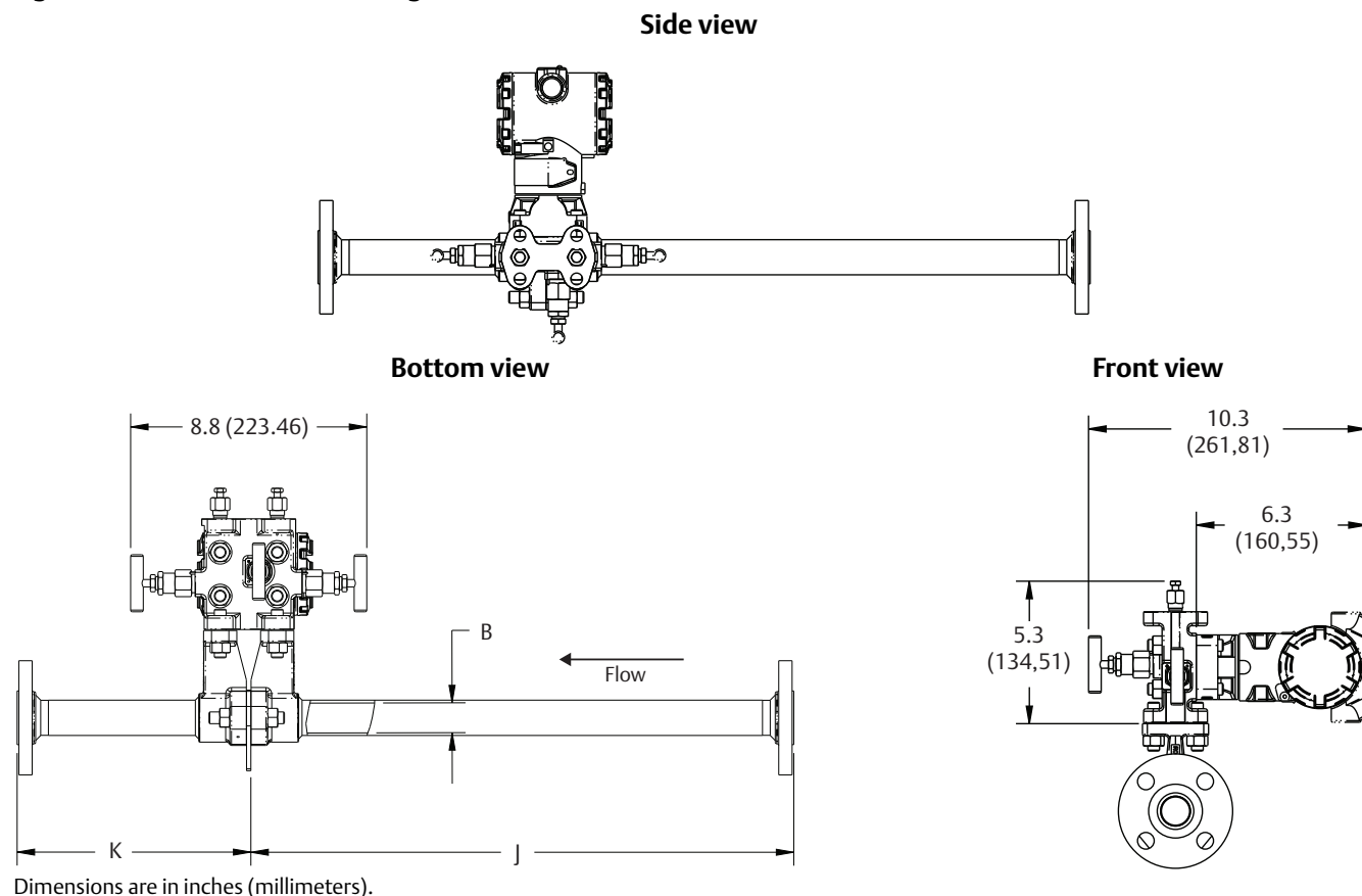
Figure 26. Rosemount 3051 CFP Integral Orifice Flowmeter
