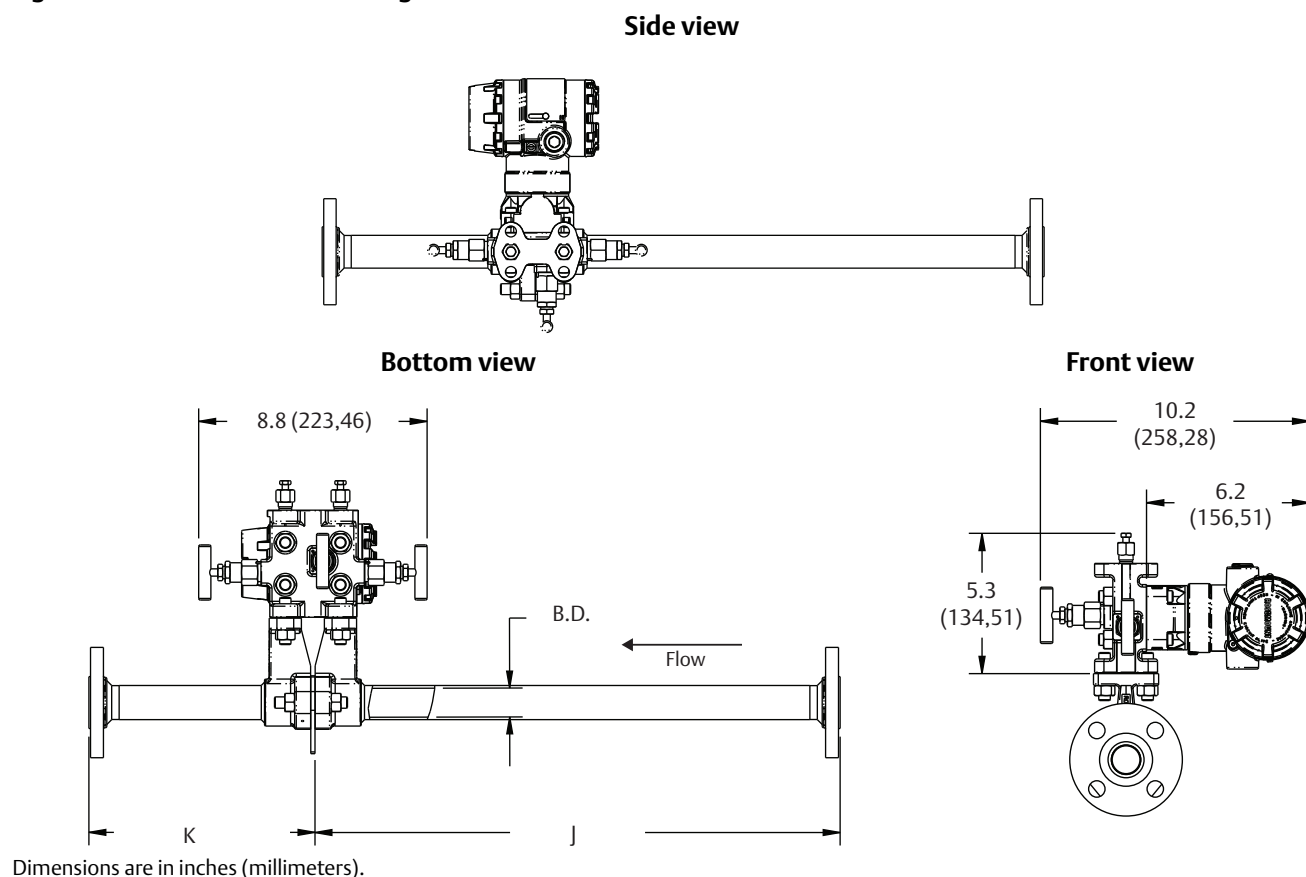
Figure 30. Rosemount 2051CFP Integral Orifice Flowmeter
