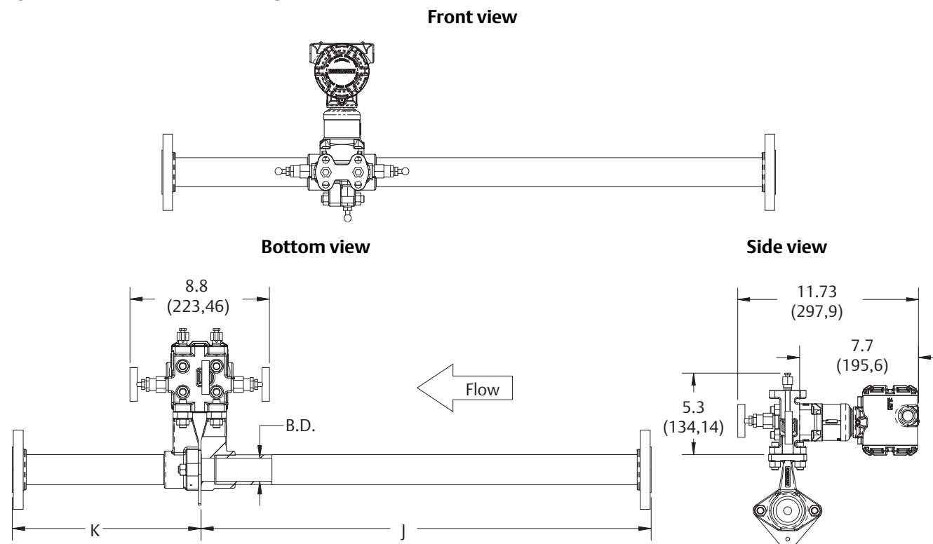
Figure 19. Rosemount 3051SFP Integral Orifice Flowmeter
