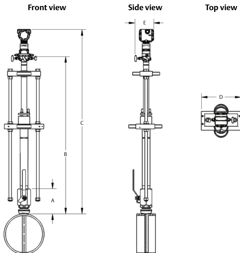
Figure 17. Rosemount 3051SFA Threaded Flo-Tap Annubar Flowmeter (1)
