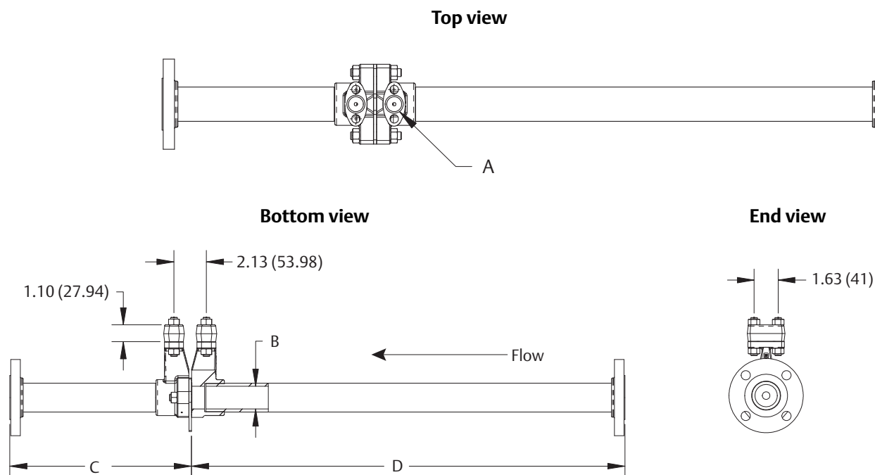
Figure 45. Rosemount 1195 Integral Orifice Plate
