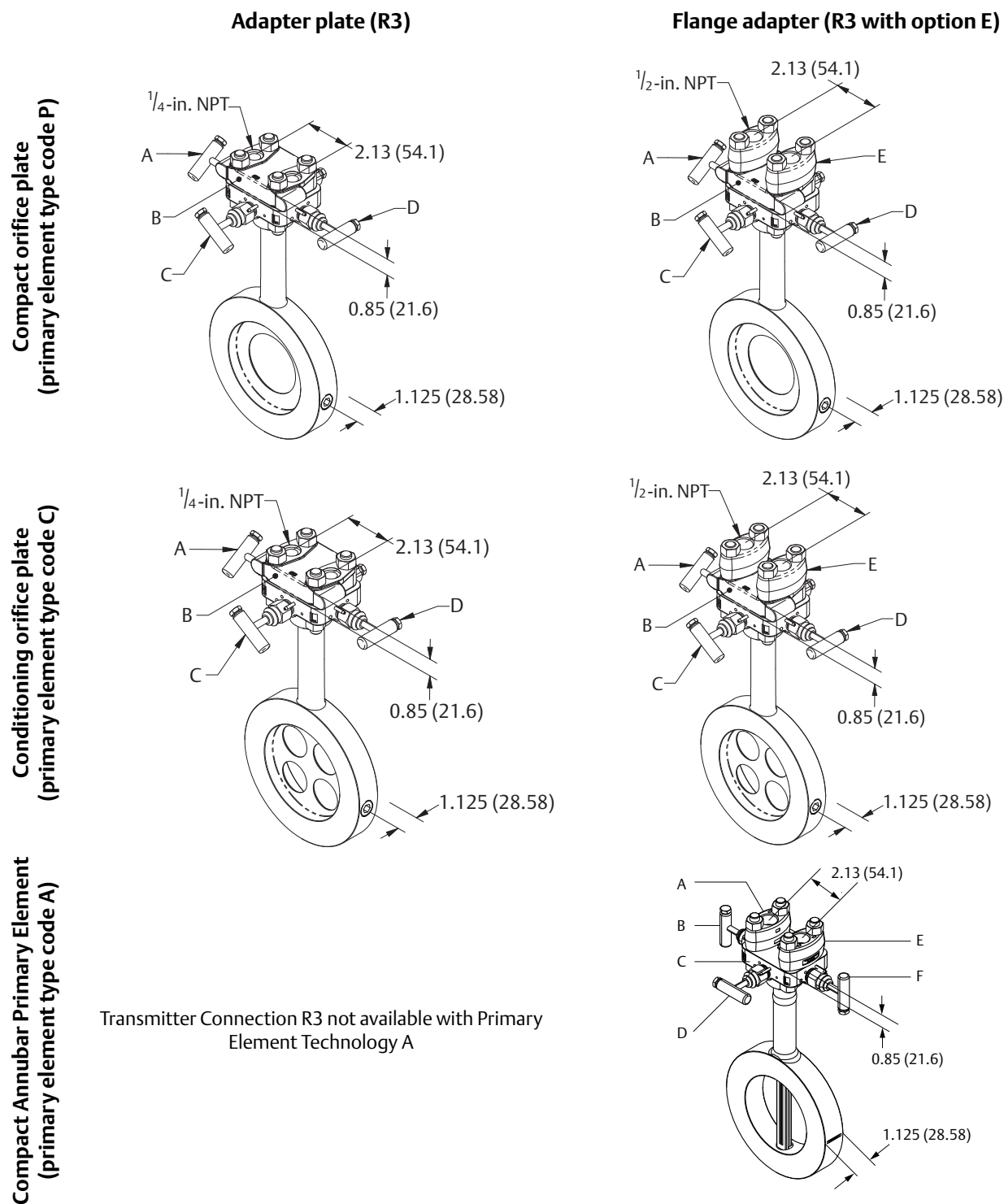
Figure 41. Rosemount 405 Compact Orifice Plate (Remote Mount Transmitter)
