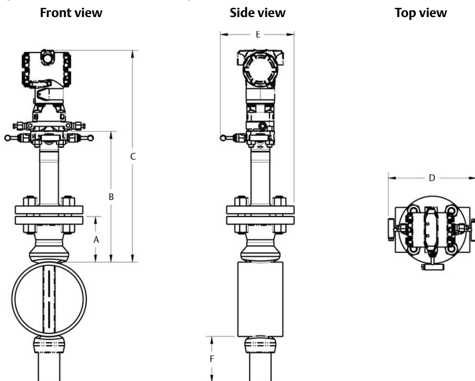
Figure 22. Rosemount 3051CFA Flanged Annubar Flowmeter
