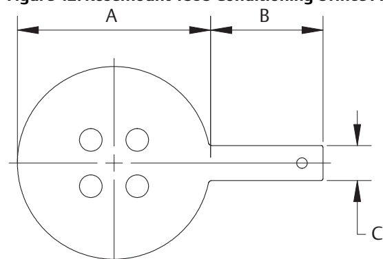
Figure 42. Rosemount 1595 Conditioning Orifice Plate (ANSI Flange, Paddle, Square Edged)
