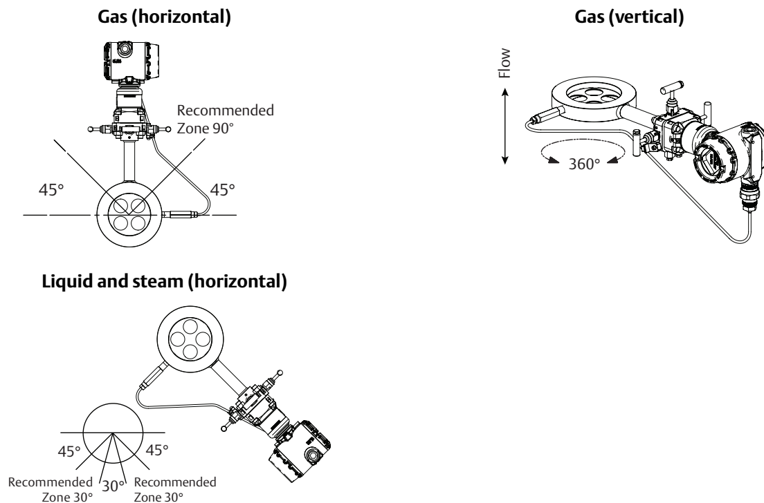
Figure 9. Rosemount 405 Direct Mount Flowmeter Orientation (Recommended)
