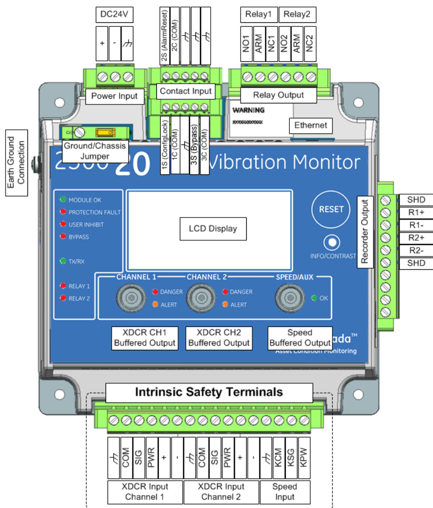
Figure 13: 2300/20 Wiring Diagram
