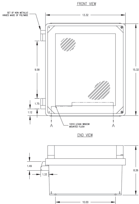
Figure 2: 105M6193-01 Weatherproof Housing
