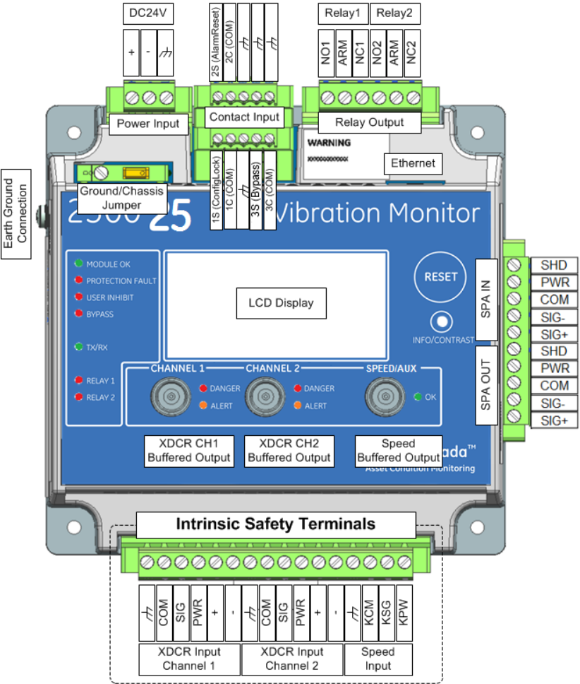
Figure 14: 2300/25 Wiring Diagram
