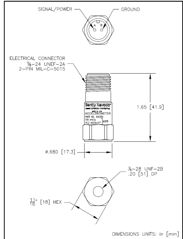
Figure 3: 200350 Accelerometer Sensor
