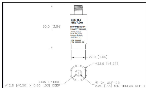
Figure 7: 330505 Velomitor
