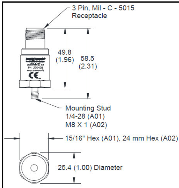
Figure 5: 330400/330425 Accelerometer Sensor
