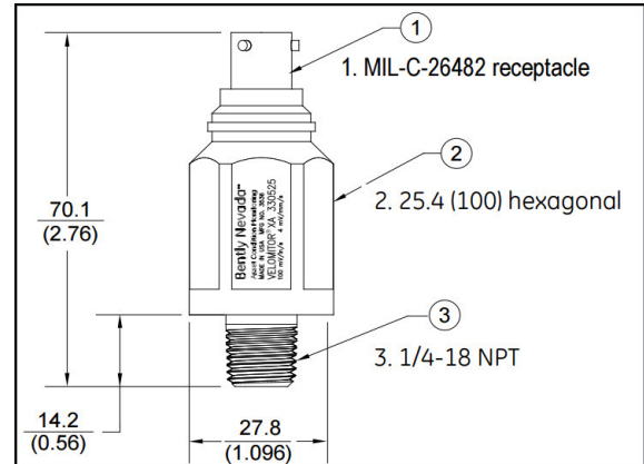
Figure 8: 330525 Velomitor
