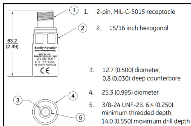
Figure 6: 330500 Velomitor
