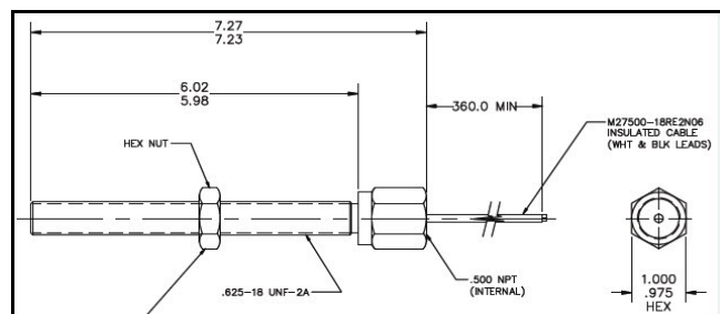
Figure 11: 284947 Magnetic Pickup
