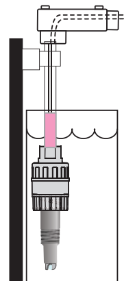
⑧ Sensor submersible installation
