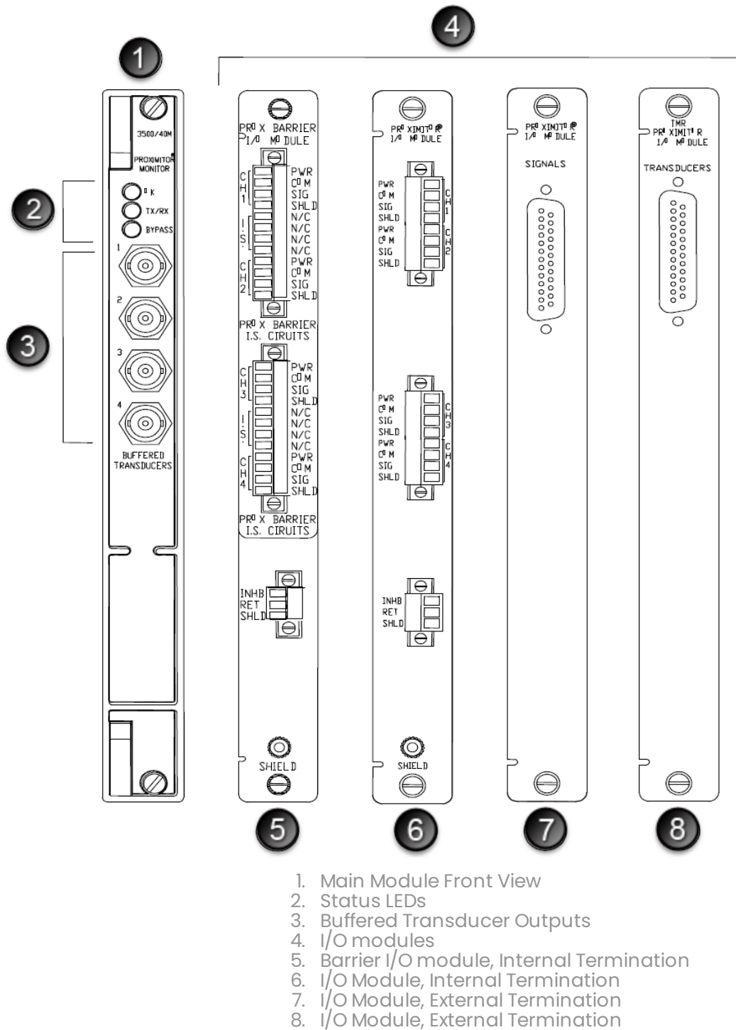
Figure 1: Assorted 3500/40M Proximito Monitor Views
