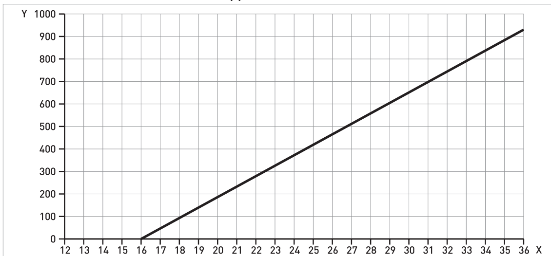
Figure 2-6: Minimum power supply voltage for an output of 21.5 mA at the terminal (Hazardous Location approval (Ex d / XP/NI))
