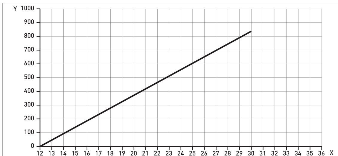
Figure 2-5: Minimum power supply voltage for an output of 21.5 mA at the terminal (Non-Ex and Hazardous Location approval (Ex i / IS))
