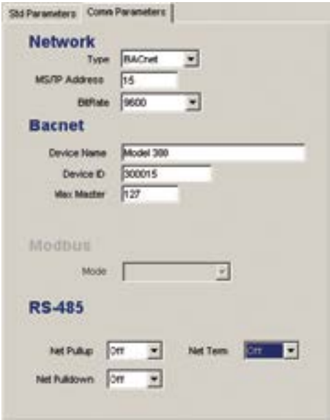
Figure 5: Comm parameters—BACnet
