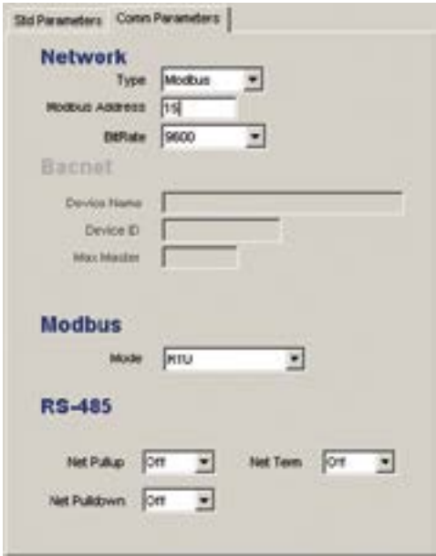
Figure 4: Comm parameters—modbus
