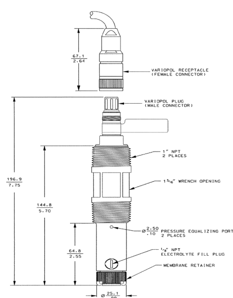
Figure 2. Rosemount 499ADO with Variopol Cable Connection Sensor Dimensions
