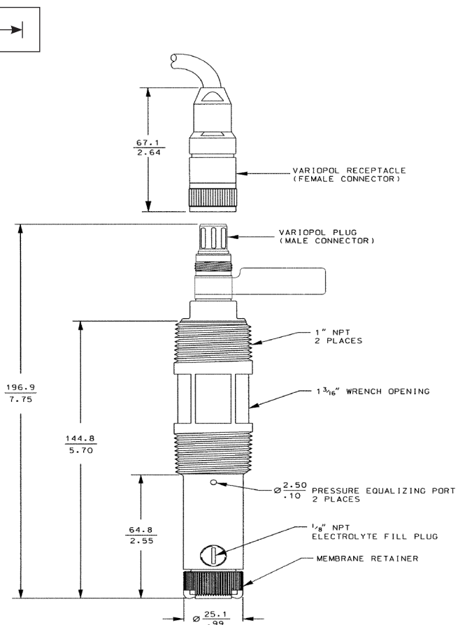
Figure 2. Sensor with Variopol connector
