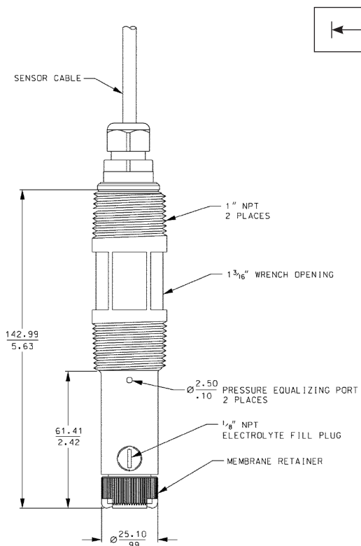
Figure 1. Standard sensor with integral cable
