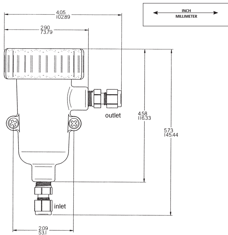
Figure 3. Low Flow Cell (PN 24091-00)
