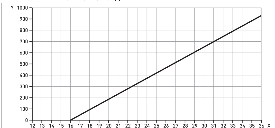
Figure 2-2: Minimum power supply voltage for an output of 21.5 mA at the terminal (Hazardous Location approval (Ex d / XP/NI))
