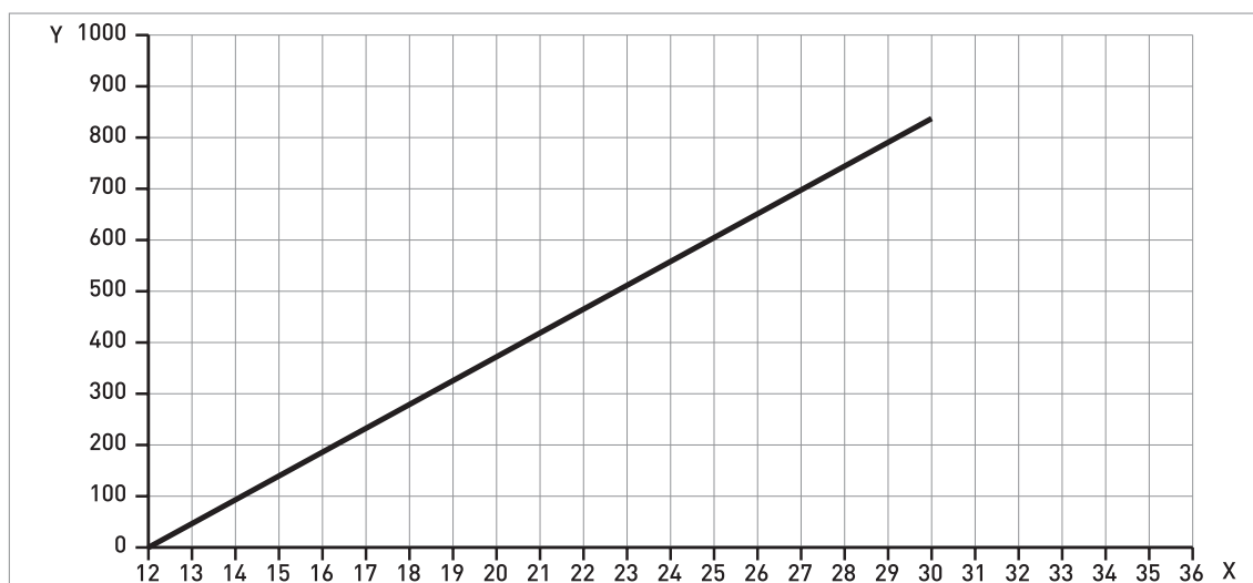
Figure 2-1: Minimum power supply voltage for an output of 21.5 mA at the terminal (Non-Ex and Hazardous Location approval (Ex i / IS))
