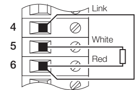
H – 2-wire RTD & Resistance
