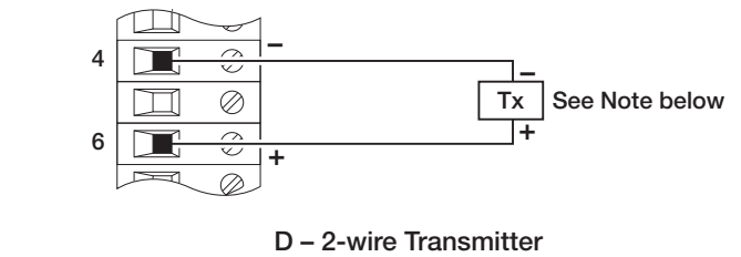
D – 2-wire Transmitter
