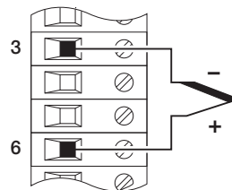
E – Thermocouple
