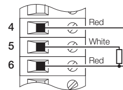
G – 3-wire RTD
