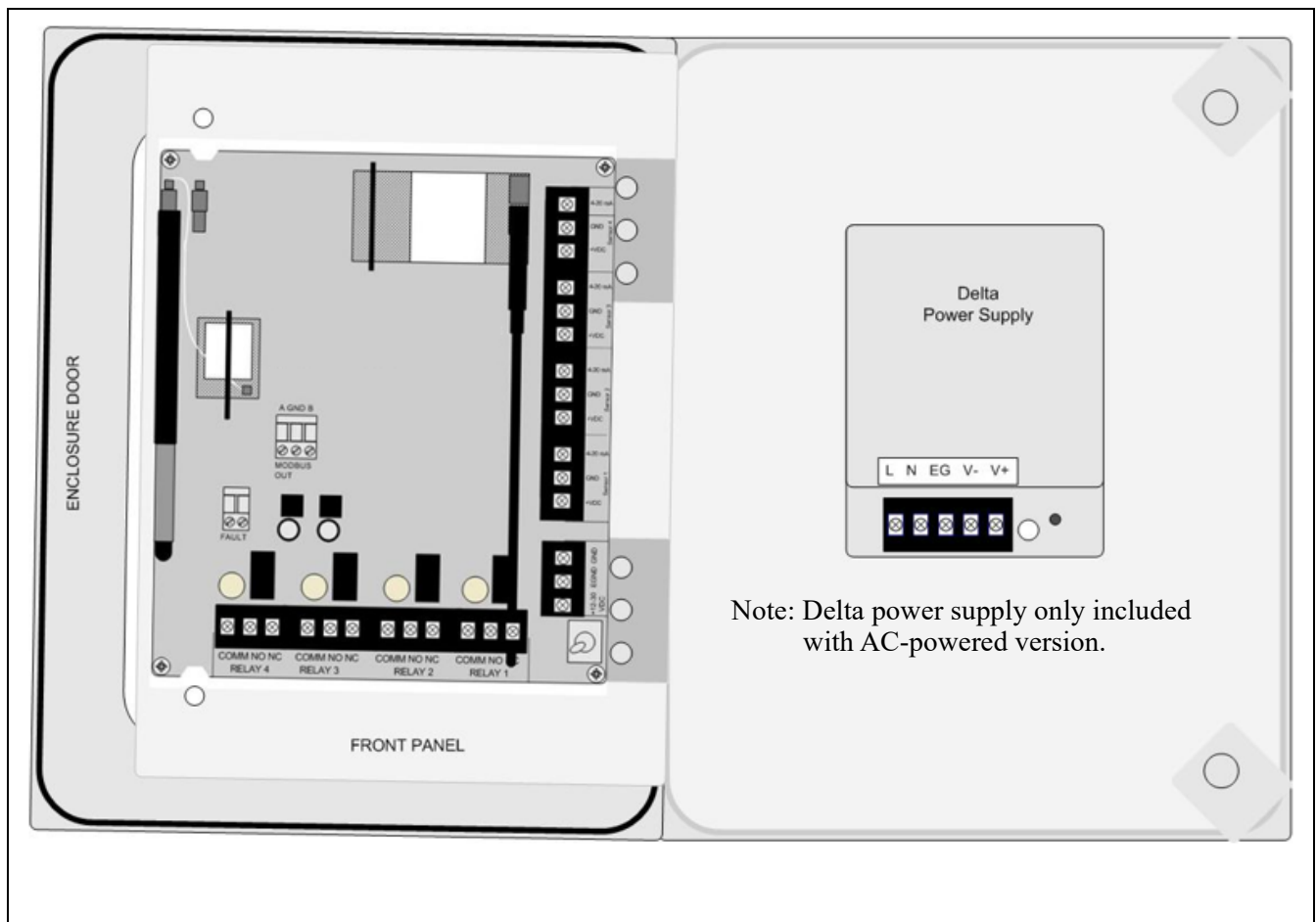
Figure 3: Internal Components
