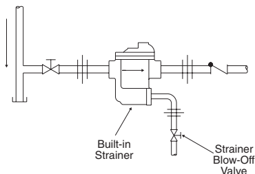
Fig. 3-4. No. 880-883 with strainer blow-down valve.
