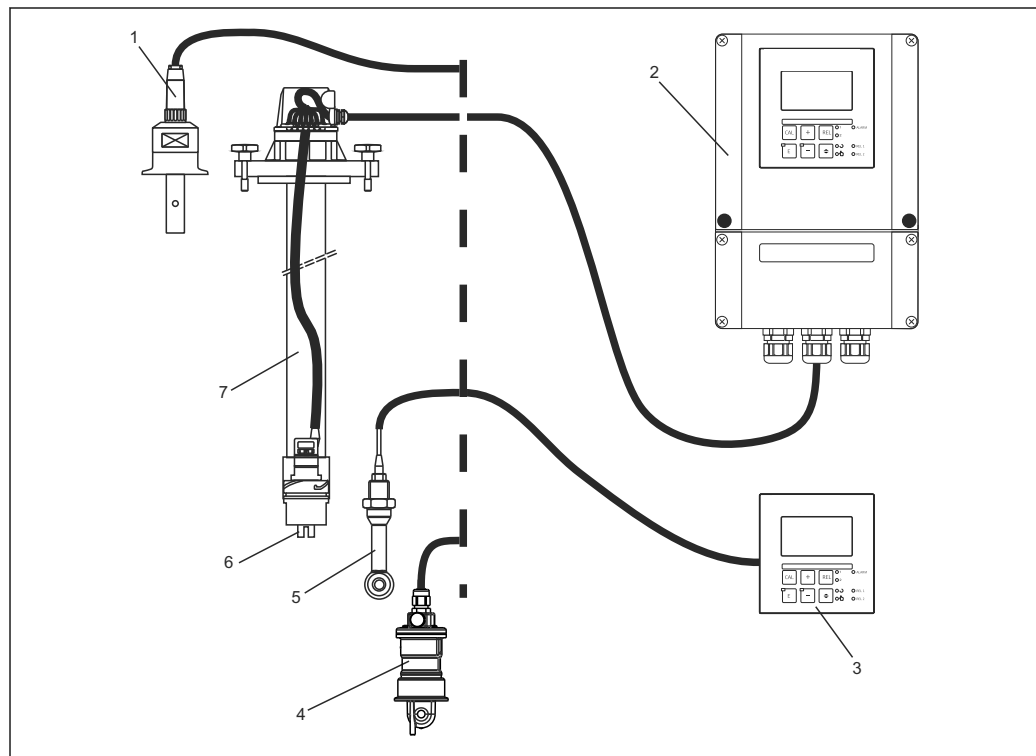
1 Complete measuring systems
