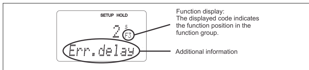
20 Information for the user on the display
