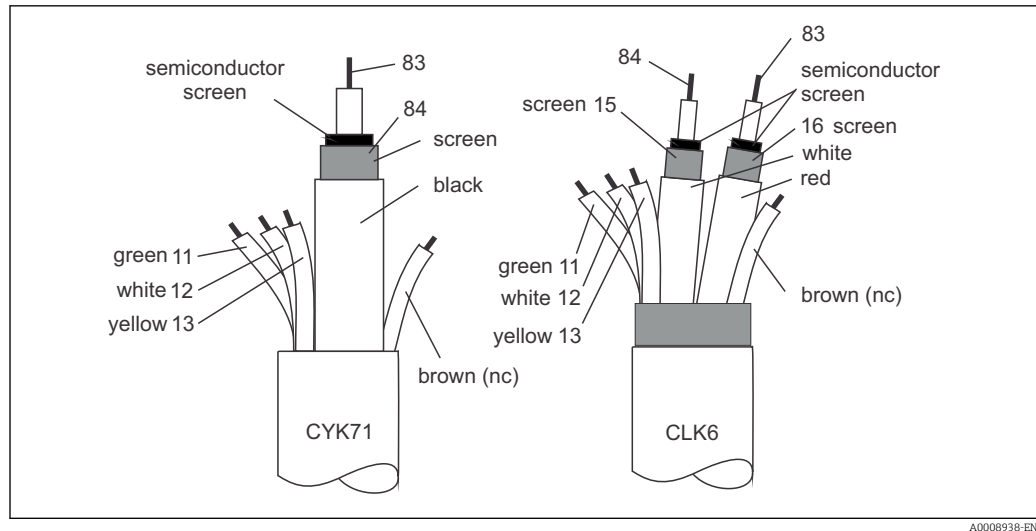
12 Structure of the special measuring cables
