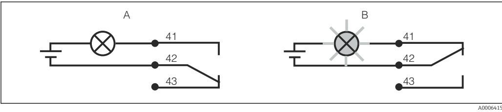
15 Recommended fail-safe switching for the alarm contact
