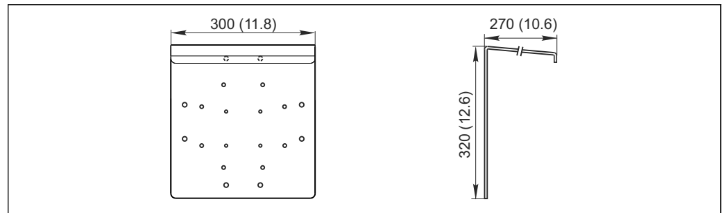
41 Dimensions in mm (inch)
