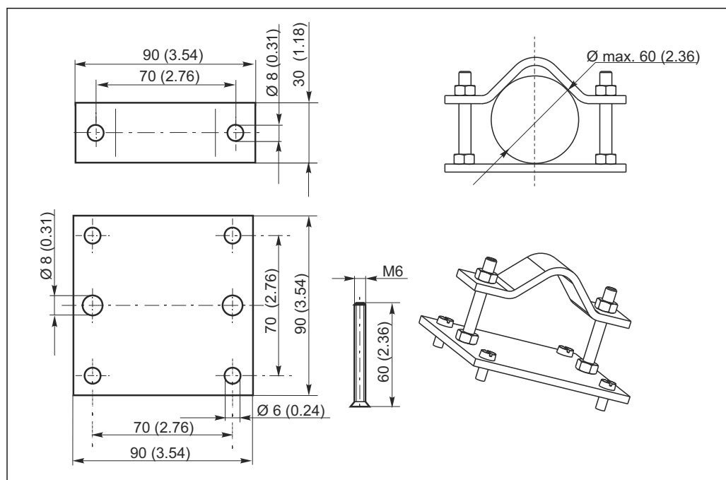
42 Dimensions in mm (inch)
