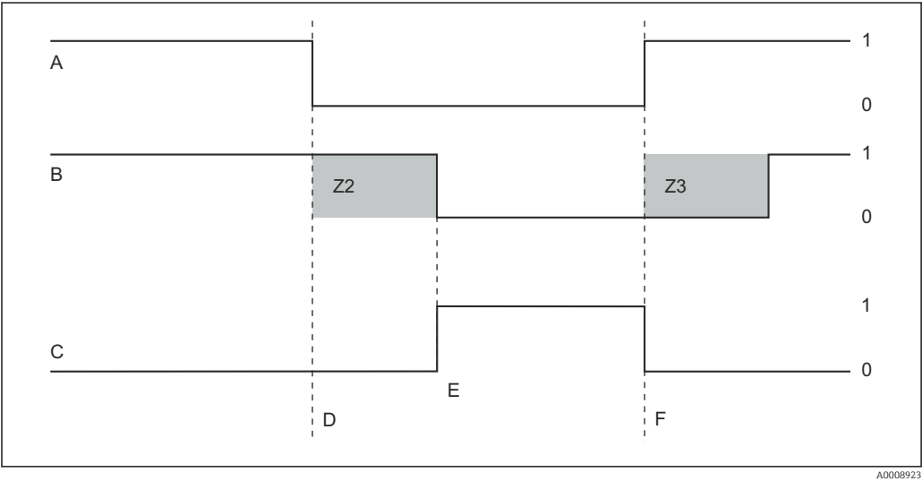
25 Alarm signaling and dosing switch-off by the main stream
