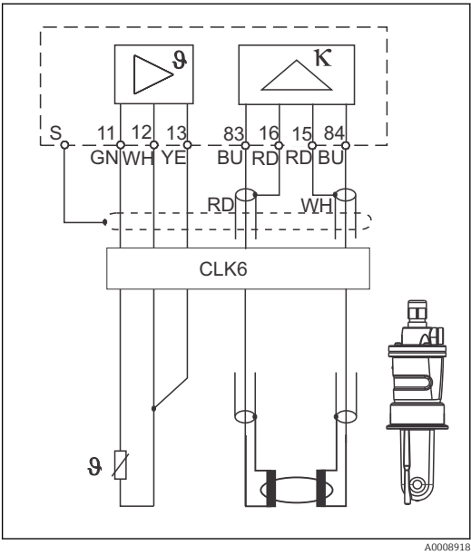
14 Connection of inductive sensors
