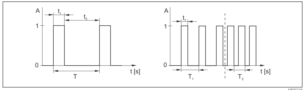
32 Signal of a pulse-length modulated controller contact (left) and of a pulse frequency-modulated controller contact (right)
