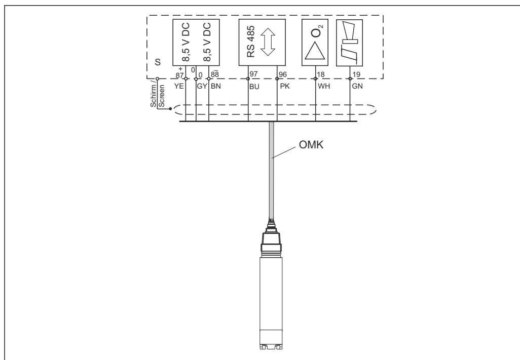
18 Connection of COS31/71 with an OMK cable
