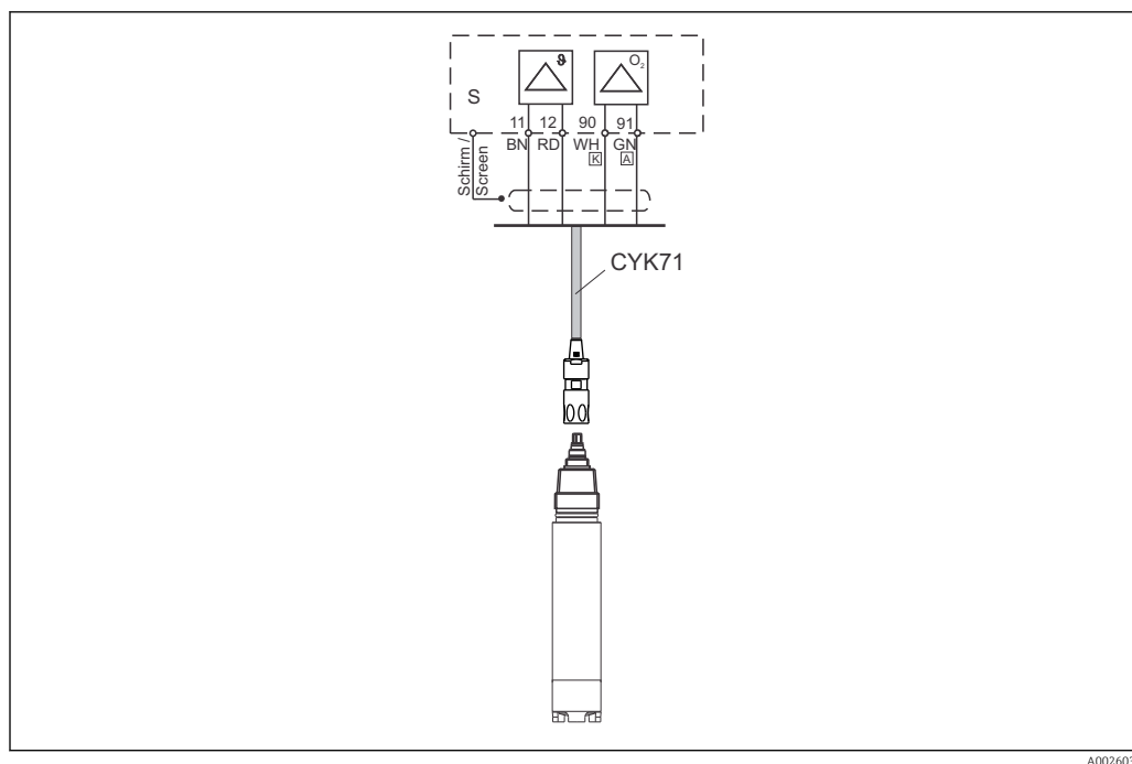
13 Connection of the COS41 with the CYK71 cable
