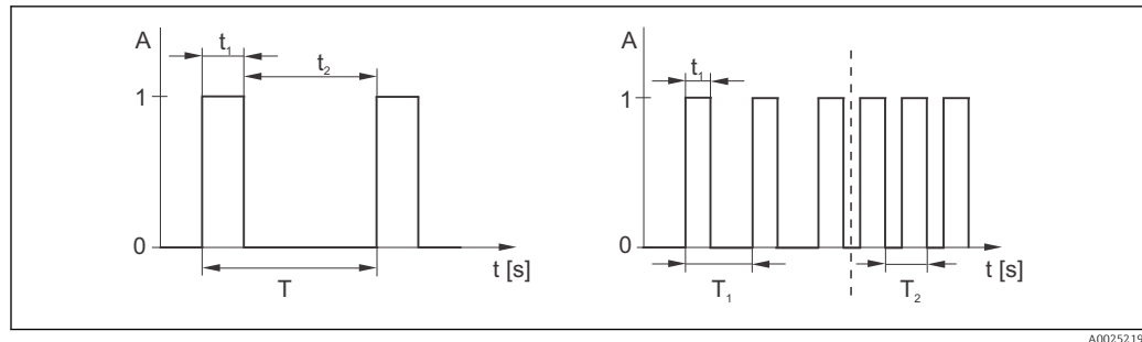
33 Signal of a pulse-length modulated controller contact (left) and of a pulse frequency-modulated controller contact (right)
