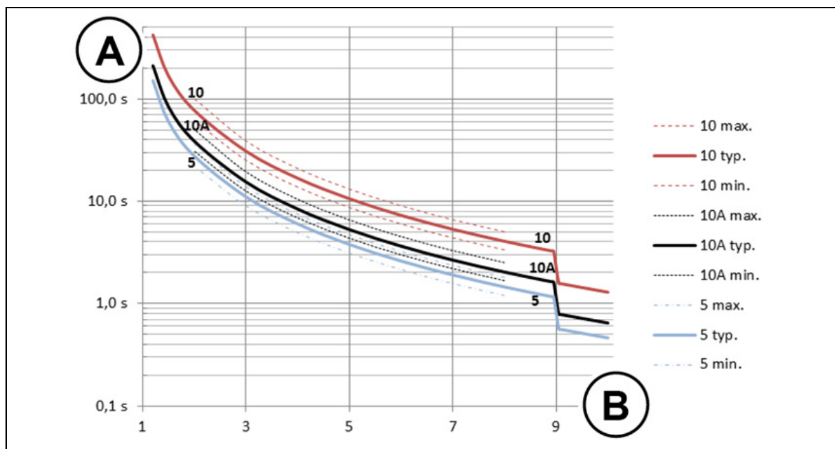
Figure 1: Trigger class curves
