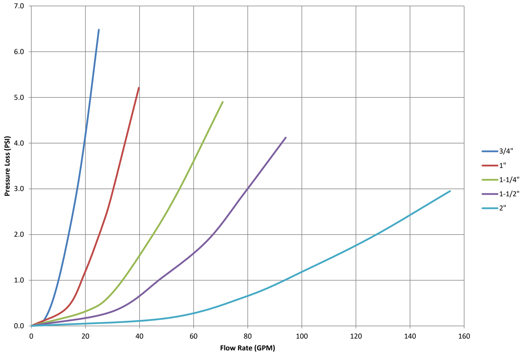
380 Btu - Pressure Loss vs. Flow Rate
