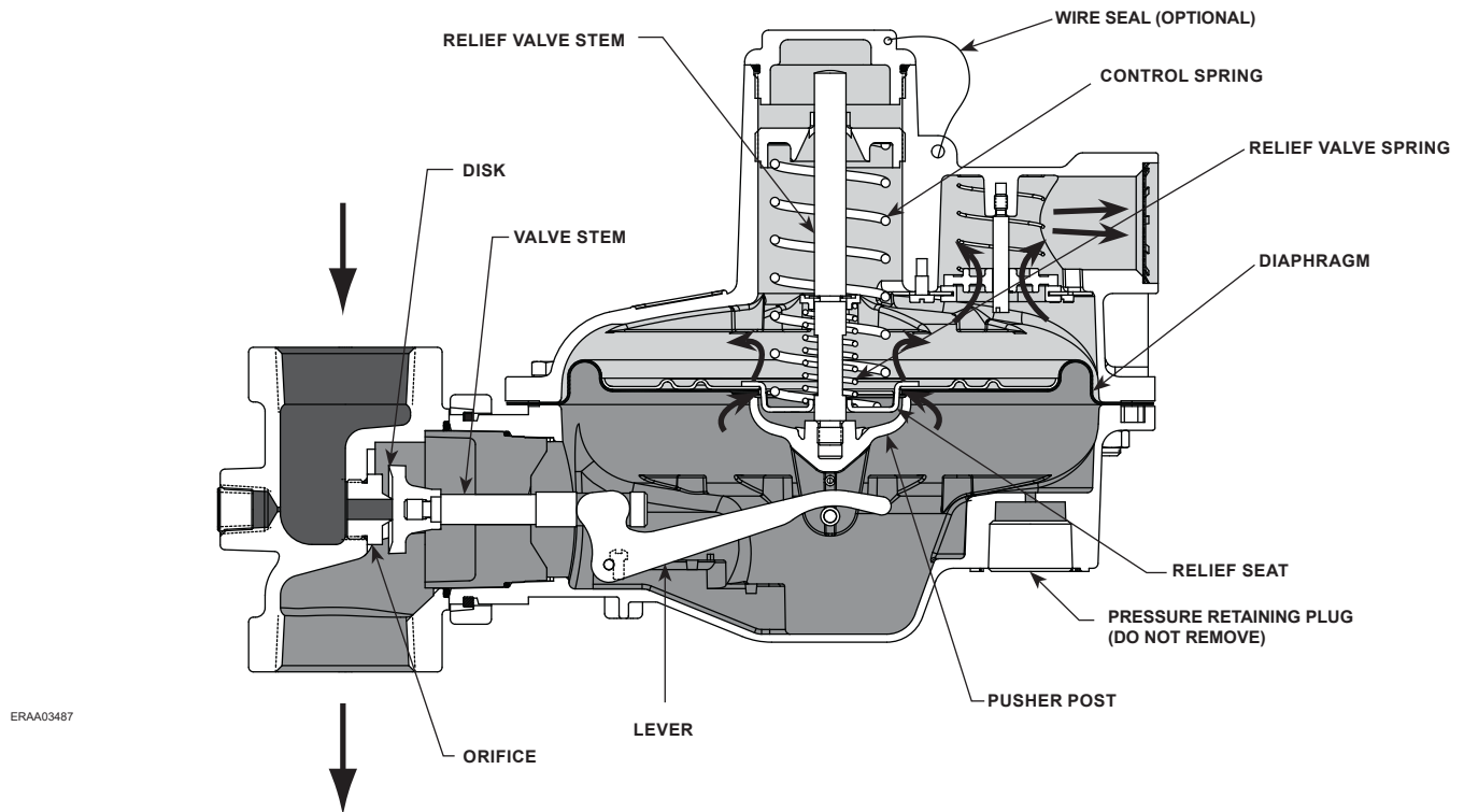
Figure 2. Type CS200IR Pressure Reducing Regulator with Internal Relief Operational Schematic
