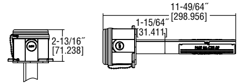
Duct Mount
