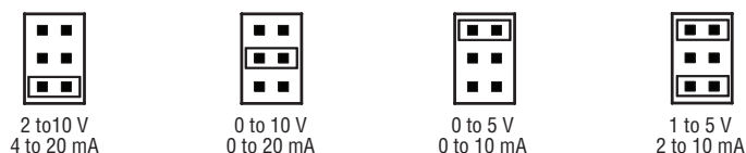
Figure 4: Output Range Selection Jumper (PJ5)
