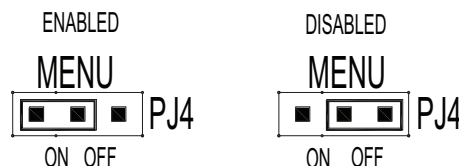
Figure 6: Menu Lockout Jumper
