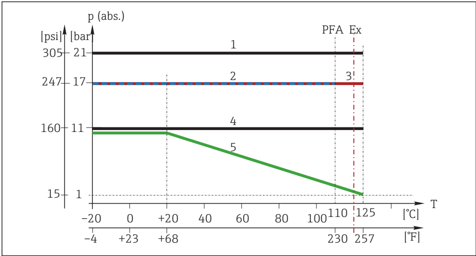
11 Pressure temperature ratings CLS50D
