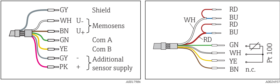
9 CYK11 for extension of CLS50D
