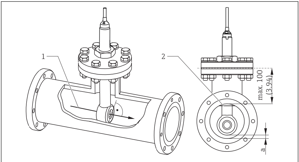
1 Sensor orientation, dimensions in mm (in)
