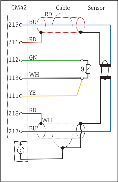
8 CLS50 to CM42
