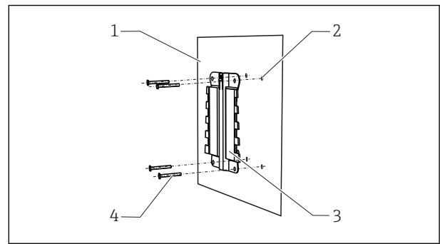
16 Wall mounting
