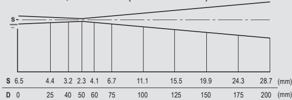
Optics CT LT CF, D:S = 22:1 (far field = 1.5:1)
