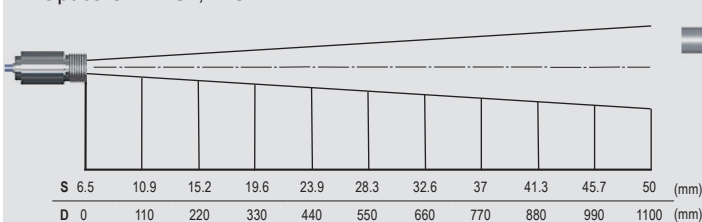
Versions with built-in CF lenses Optics CT LT SF, D:S = 22:1
