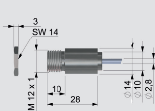
Sensing head (standard)
