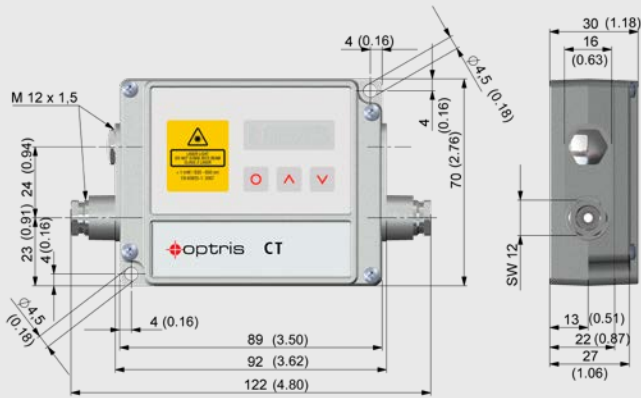
Electronics
