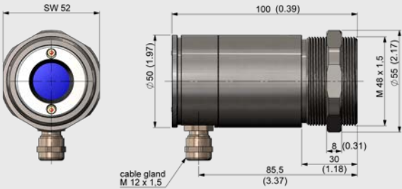
Sensing head
