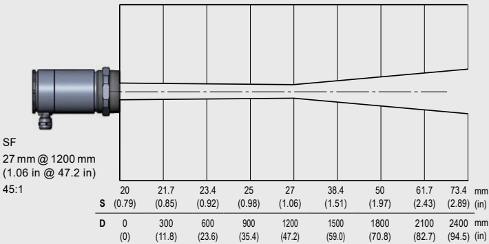
Chart SF optics, D:S = 45:1
