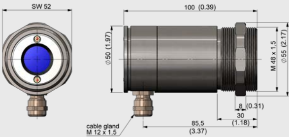
Sensing head
