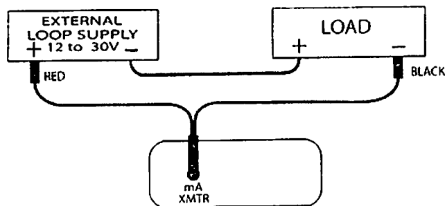
Fig 3. Simulate a 2-Wire mA Transmitter Loop With External 12 to 30V DC Supply. A similar connection can be used to extend output range of CSG beyond 300 ohms. A 24V source will allow CSG to source into an impedance of >1000 ohms.
