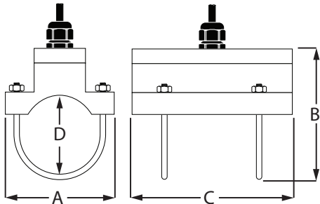
Fixed Small Pipe U-Bolt Connections CF, CL ANSI/DN and Copper 2 in. Models (Not for metric pipes.)
