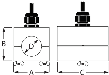
Fixed Small Pipe Pipes and Tubing 1/2...2 in. (Not for metric pipes.)
