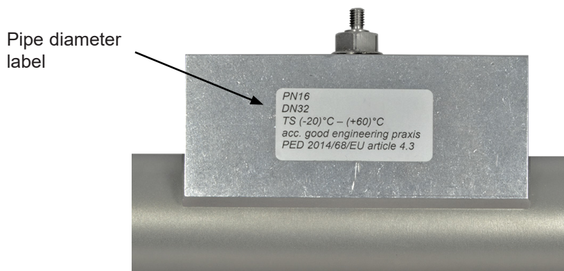
Fig. 2 Pipe diameter on gauge mounting block with flanges
