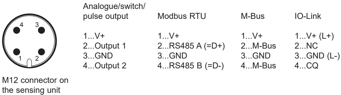
Fig. 12 M12 connector
