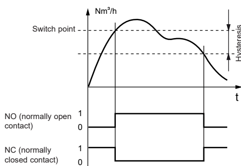
Fig. 3 Hysteresis mode
