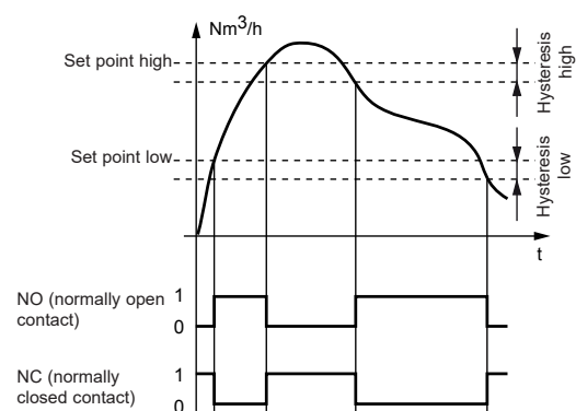
Fig. 4 Window mode
