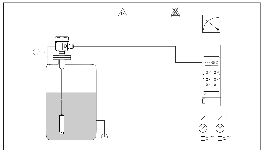
1 Level measurement
