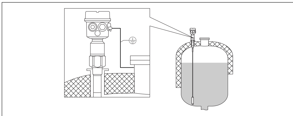
4 A probe with inactive length for the insulated tanks
