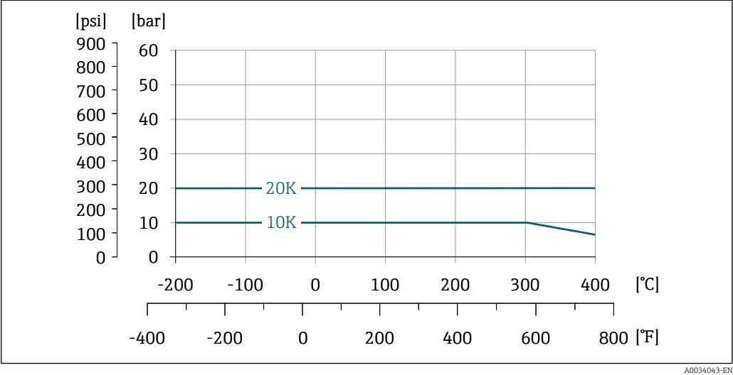
22 Flange connection material: stainless steel, multiple certifications, 1.4404/F316/F316L
