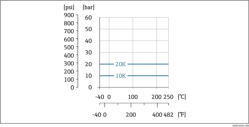
23 Flange connection material: cast, CX2MW similar to Alloy C22/2.4602
