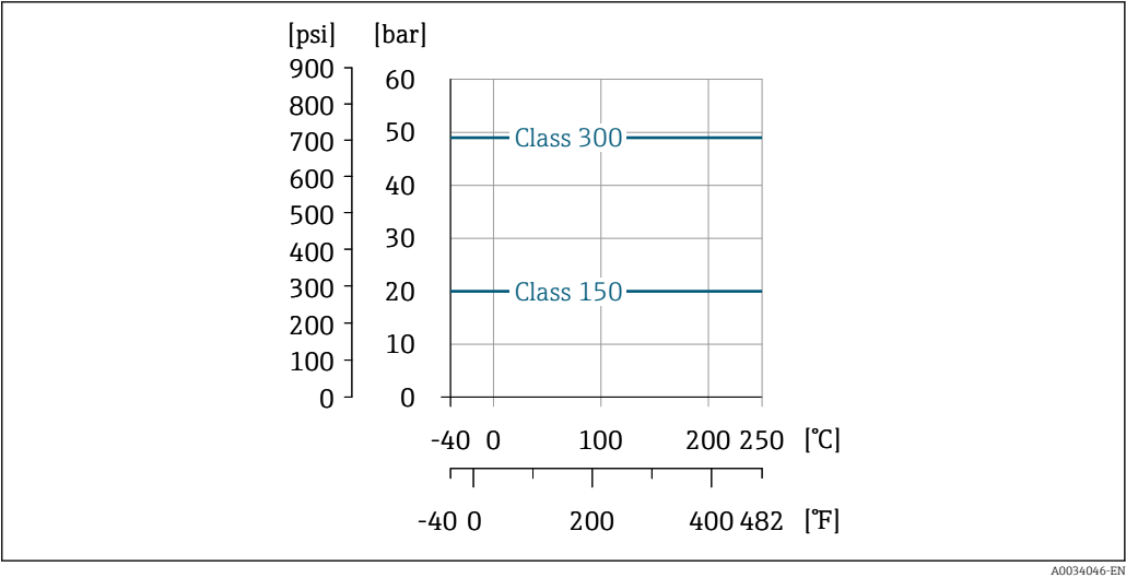
21 Flange connection material: cast, CX2MW similar to Alloy C22/2.4602
