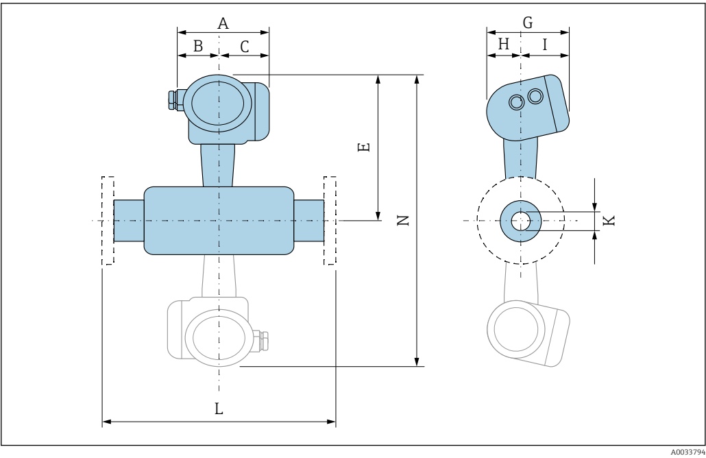
24 Grayed out: Dualsens version
