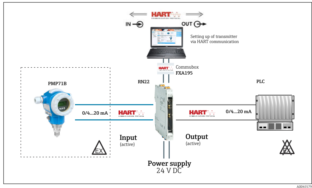
17 Pressure measurement in a hazardous area with an RN22 active barrier
