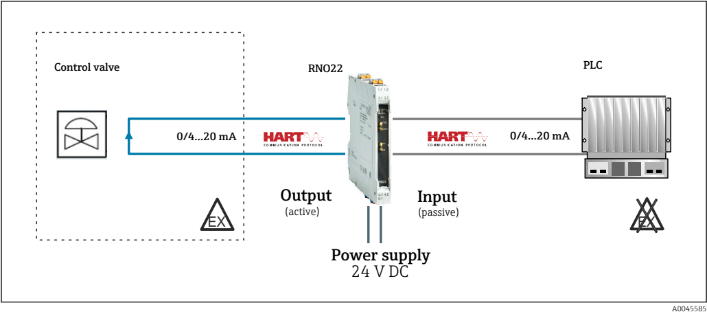
23 Control valve activation in the hazardous area with an RN022 output isolating amplifier
