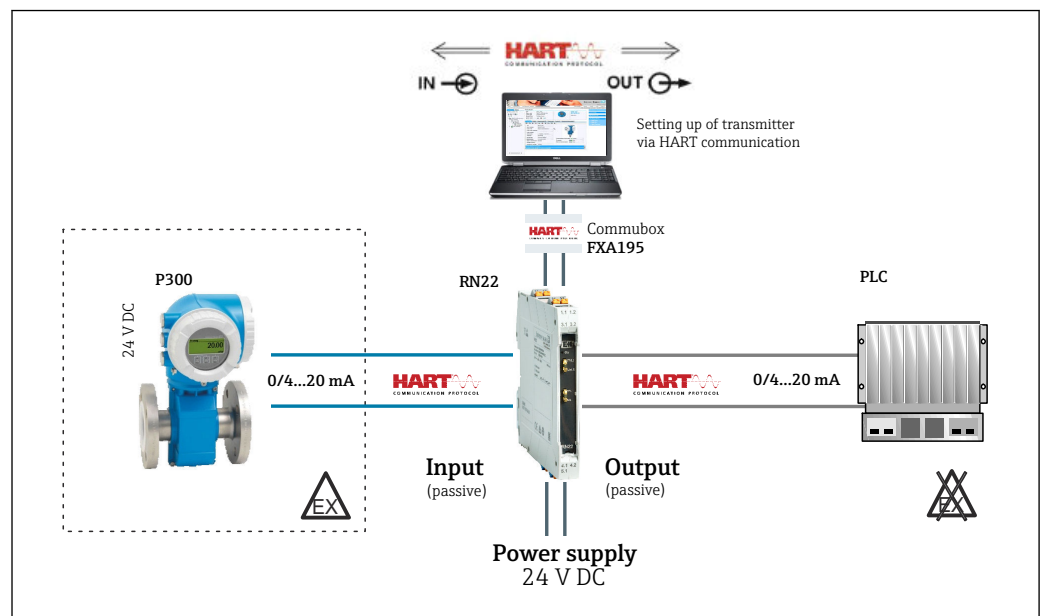
18 Flow measurement in the hazardous area with an RN22 active barrier
