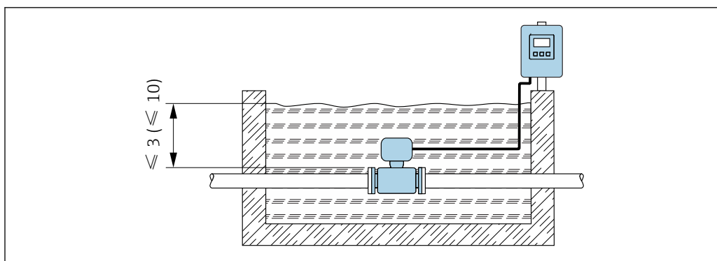
31 Engineering unit in m(ft)
