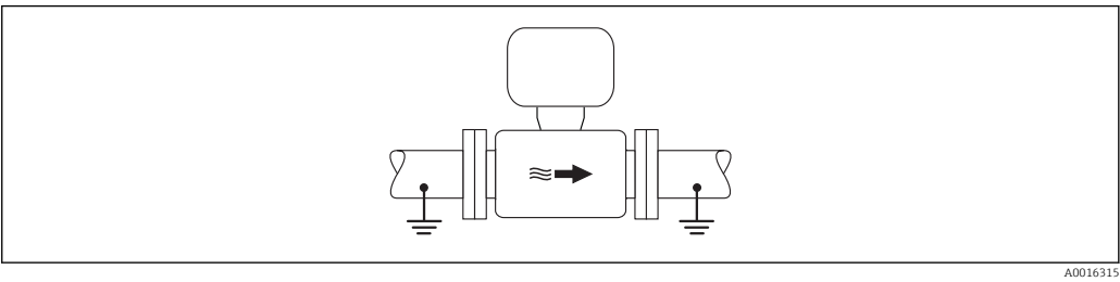
20 Potential equalization via measuring tube
