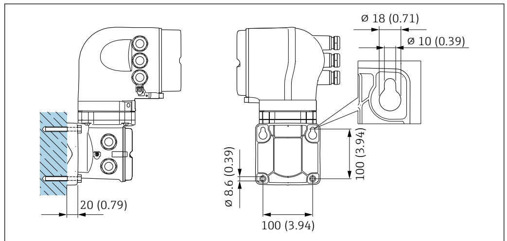
30 Engineering unit mm (in)
