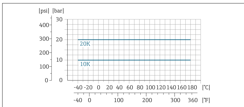
38 Process connection material: stainless steel, F316L similar to 1.4404; carbon steel, A105/A350LF2
