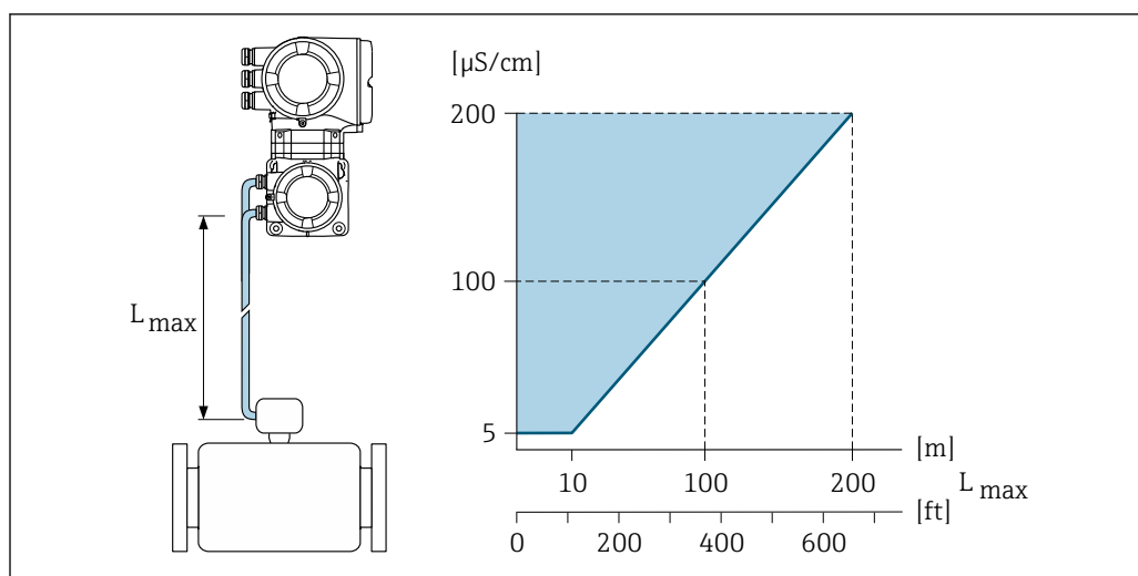
28 Permitted length of connecting cable
