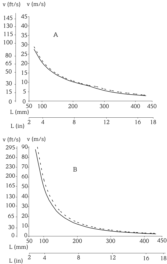
19 Maximum flow velocity with thermowell diameter 14 mm (0.55 in) (—) or 15 mm (0.6 in) (-----)
