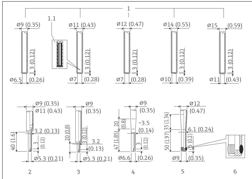
26 Available thermowell tips (reduced, straight or tapered). Maximum surface roughness R_a \leq 0.76 \mu\text{m} (30 \mu\text{in} ). Bottom thickness = 3 mm (0.12 in) for straight version, except bottom thickness for schedule (SCH) straight versions = 4 mm (0.16 in)
