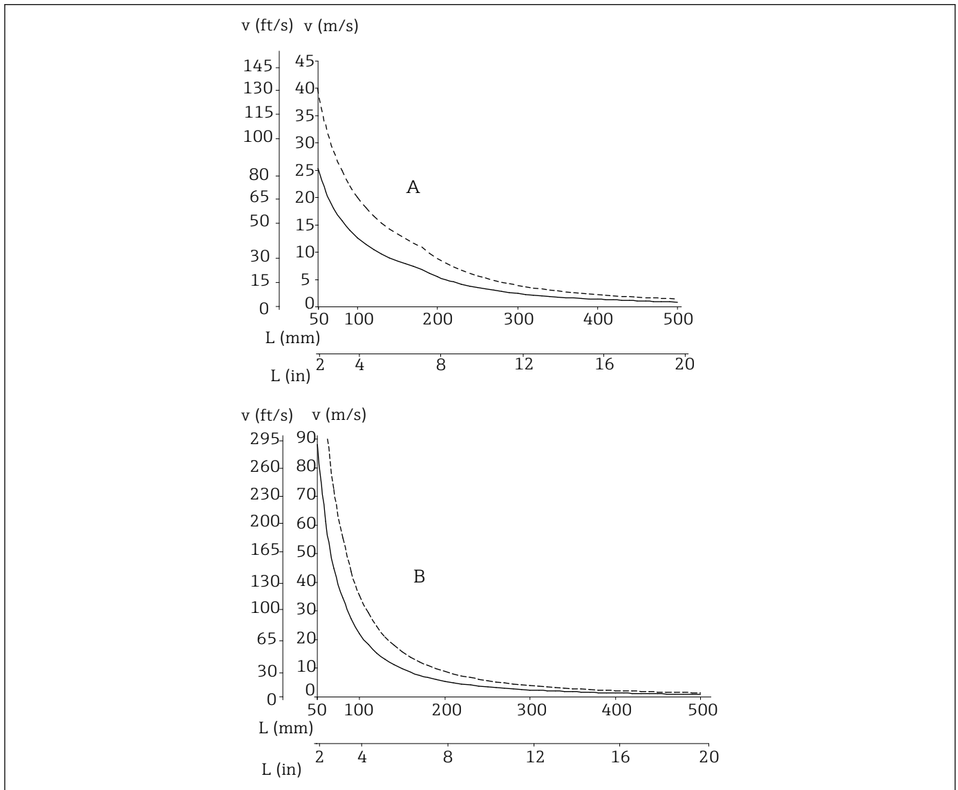
18 Maximum flow velocity with thermowell diameter 9 mm (0.35 in) (—) or 12 mm (0.47 in) (----)
