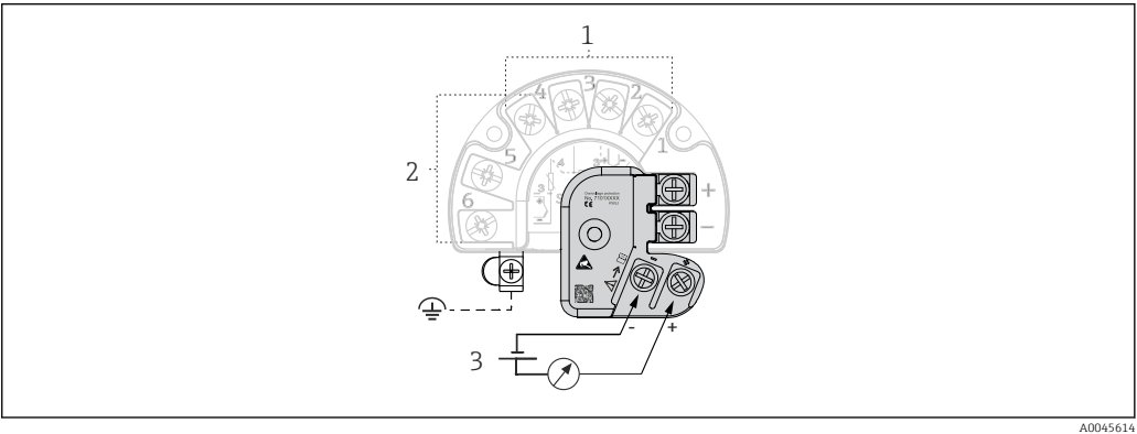
10 Electrical connection of surge arrester
