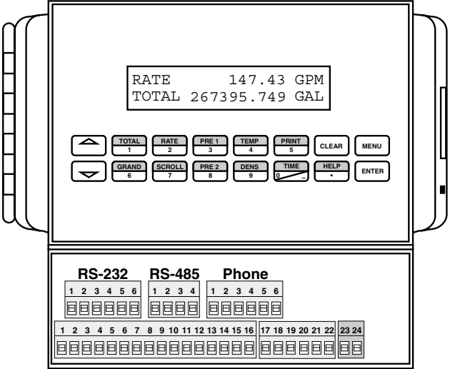
NEMA 12, 13 Terminal Layout
