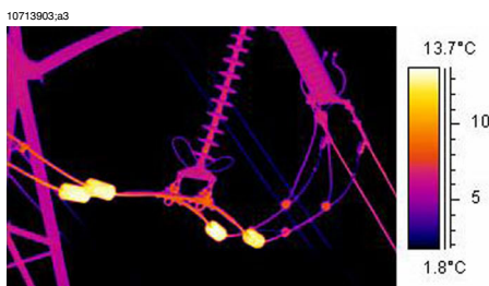
Figure 25.13 An infrared image of hot stabilizing weights
