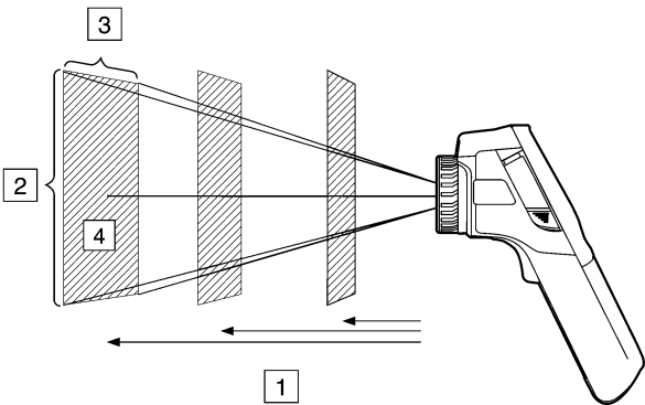
Figure 21.1 Relationship between field of view and distance. 1: Distance to target; 2: VFOV = vertical field of view; 3: HFOV = horizontal field of view; 4: IFOV = instantaneous field of view (size of one detector element).
