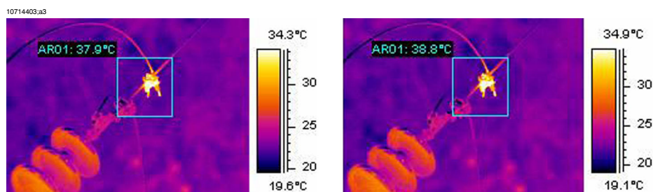
Figure 25.18 LEFT: Incorrect distance setting; RIGHT: Correct distance setting
