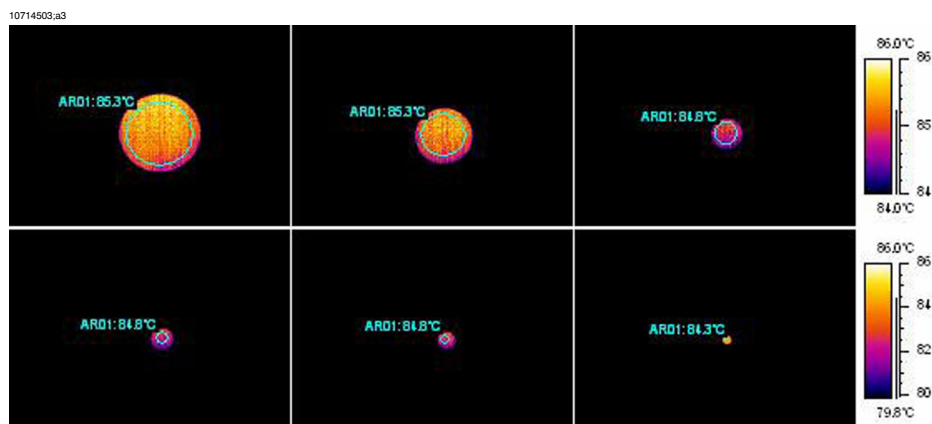
Figure 25.19 Temperature readings from a blackbody at +85^{\circ}\text{C} ( +185^{\circ}\text{F} ) at increasing distances
