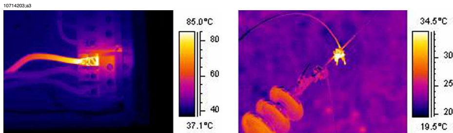
Figure 25.16 LEFT: An infrared image showing bad contact due to a loose bolt; RIGHT: A loose outdoor connection, exposed to the wind cooling effect.
