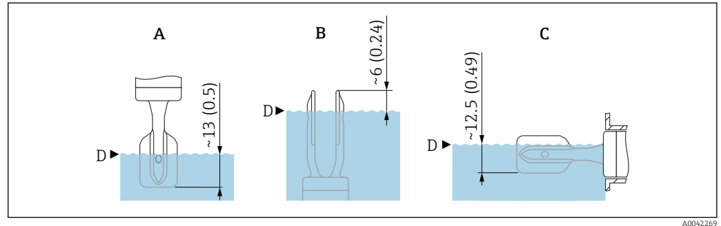
17 Typical switch points, plastic-coated tuning fork. Unit of measurement mm (in)
