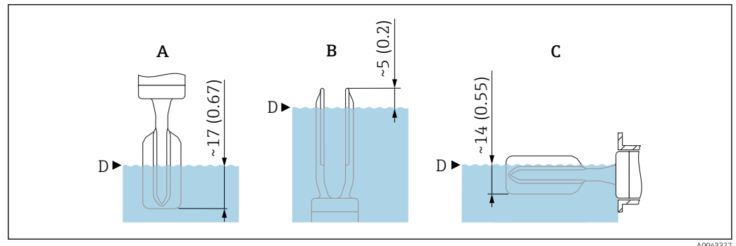
18 Typical switch points, enamel-coated tuning fork. Unit of measurement mm (in)
