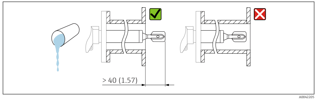
9 Installation example for a highly viscous liquid. Unit of measurement mm (in)
