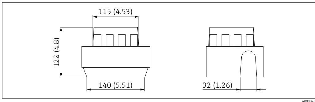
47 Protective cover for single compartment housing, aluminum or 316L. Unit of measurement mm (in)
