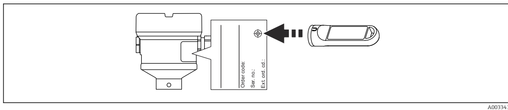
42 Functional test with test magnet
