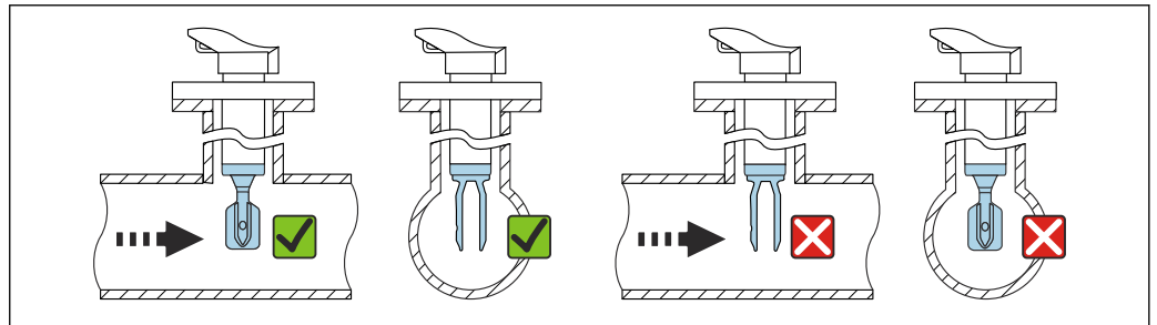
14 Installation in pipes
