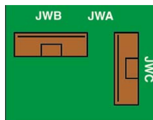
120 VAC Configuration
