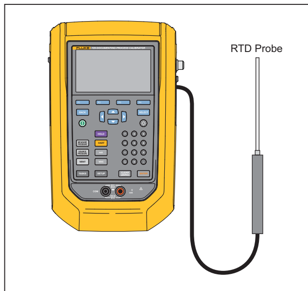
Figure 20. Temperature Probe Connection
