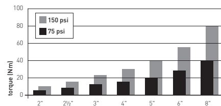
Moving torques in relation to the line pressure
