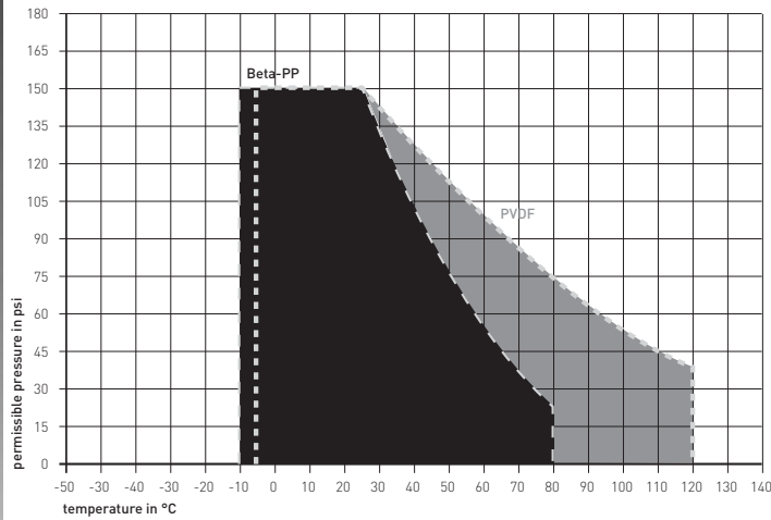
Pressure-temperature diagram PROGEF® Polypropylene, PVDF (useful life 25 years; medium water)
