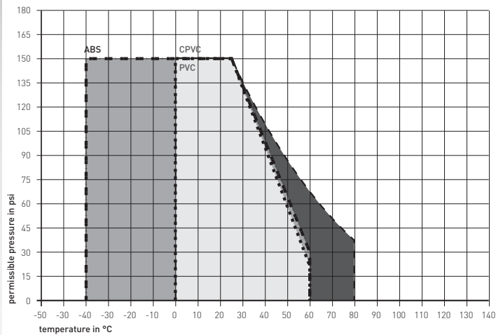
Pressure-temperature diagram ABS, PVC, CPVC (useful life 25 years; medium water)
