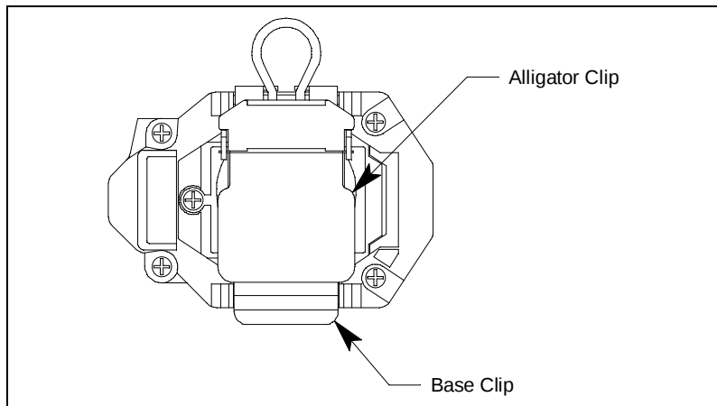
Figure 2: Alligator Clip
