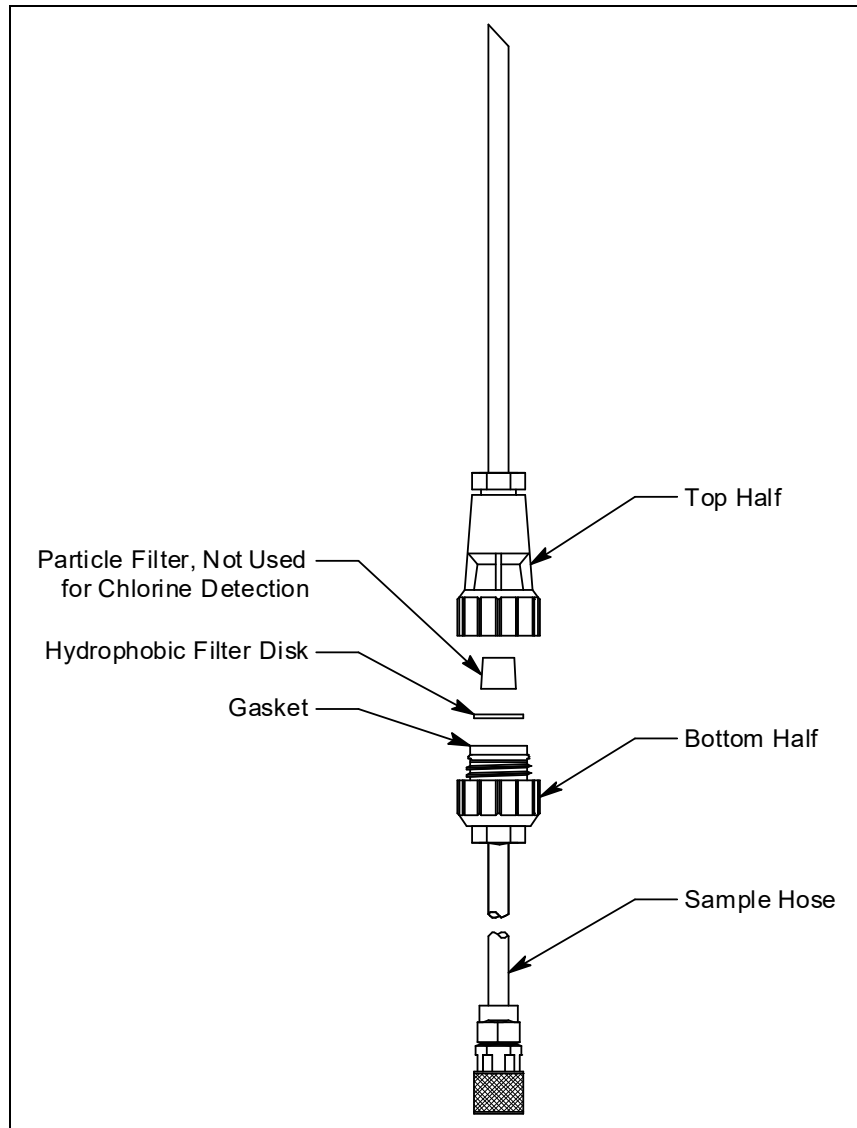
Figure 24: Replacing the Particle Filter and Hydrophobic Filter Disk
