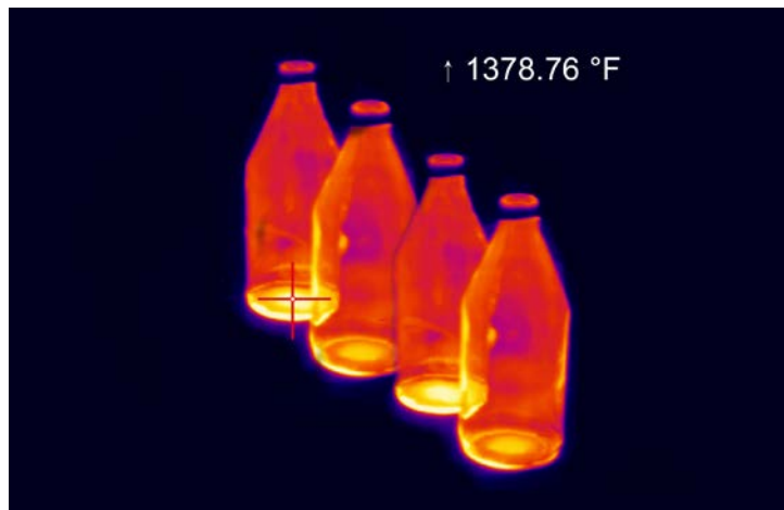
Hot spot detection at glass bottle production
