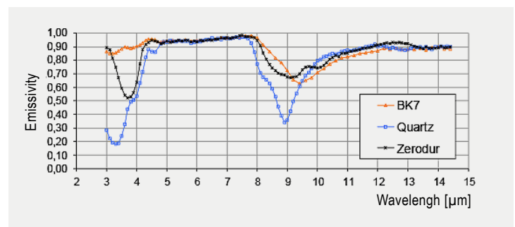
Spectral emissivity of glass
