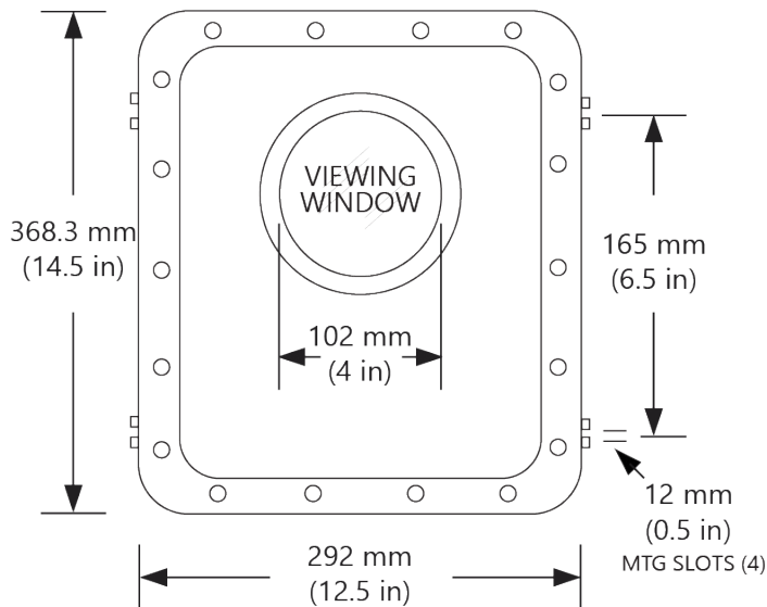
End View
