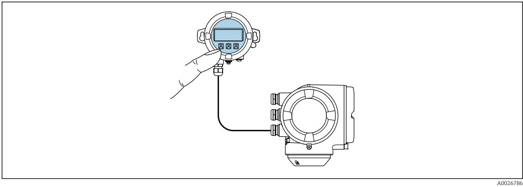
54 Operation via remote display and operating module DKX001
