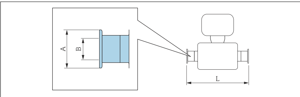
51 Hygienic clamp adapter connection suitable for pipes with connection according to ASME BPE (reduction)
