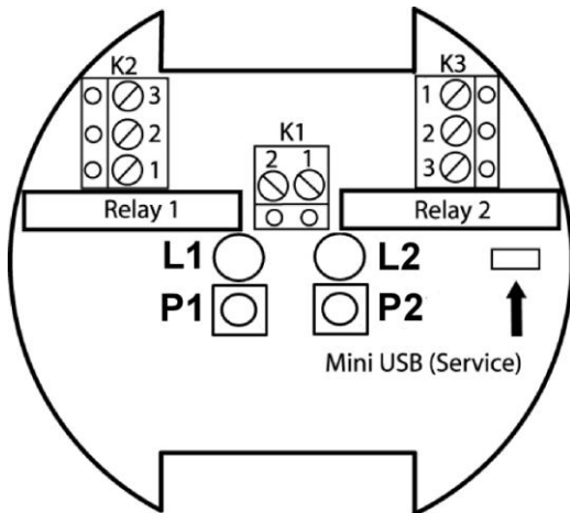
Terminal block diagram for type D and W
