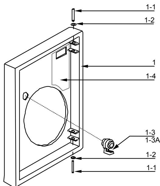
Figure 10-1 Door assembly
