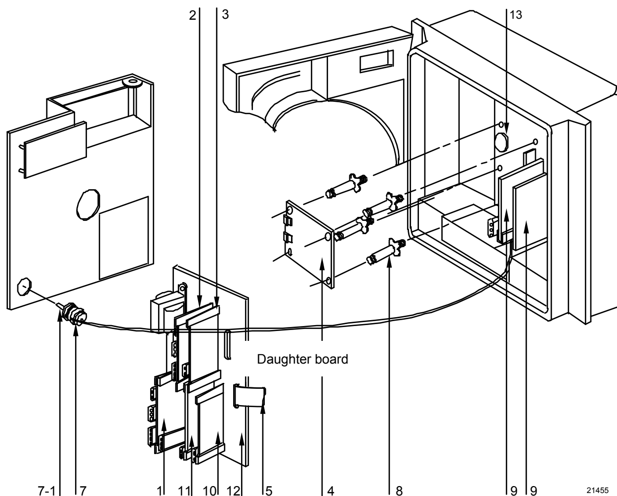
Figure 10-4 Recorder components associated with options
