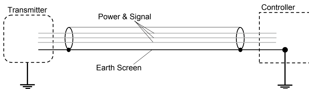
Diagram 11: System grounding
