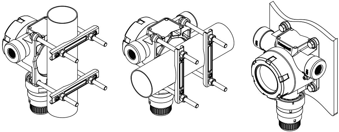
Diagram 5: Mounting arrangements
