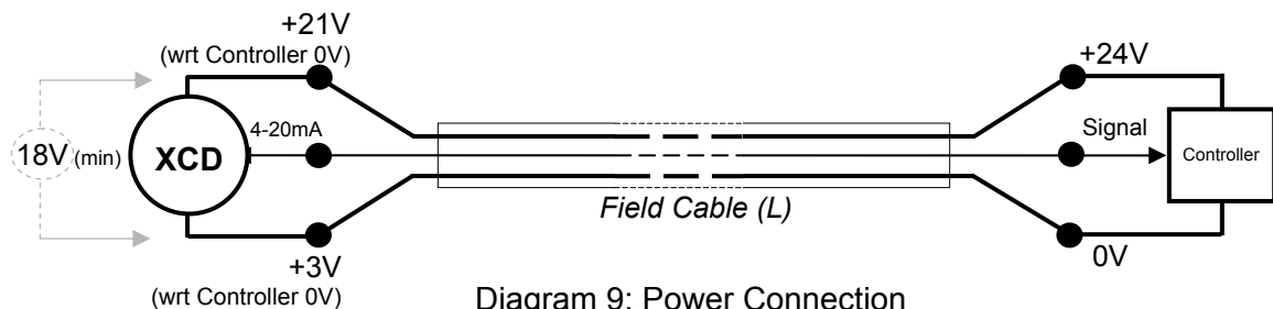
Diagram 9: Power Connection
