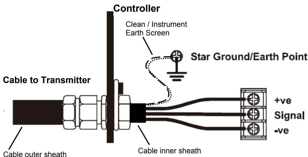
Diagram 10: Controller Grounding
