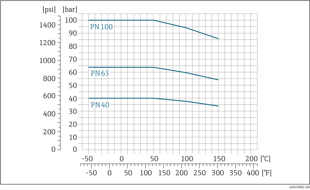
23 With flange material 1.4301 (304); wetted parts: titanium
