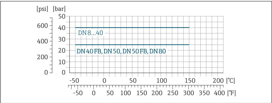
27 With connection material Grade 2 titanium
