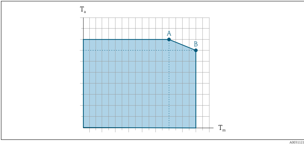
22 Exemplary representation, values in the table below. T_a Ambient temperature range T_m Medium temperature A Maximum permitted medium temperature T_m at T_{a\max} = 60\text{ °C} (140 °F); higher medium temperatures T_m require a reduced ambient temperature T_a B Maximum permitted ambient temperature T_a for the maximum specified medium temperature T_m of the sensor
