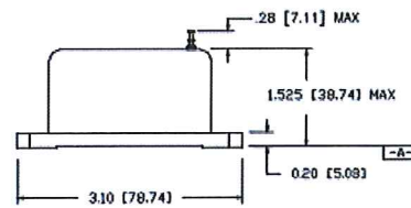
LCA-100 SERIES w/4 TURRET STYLE TERMINALS
